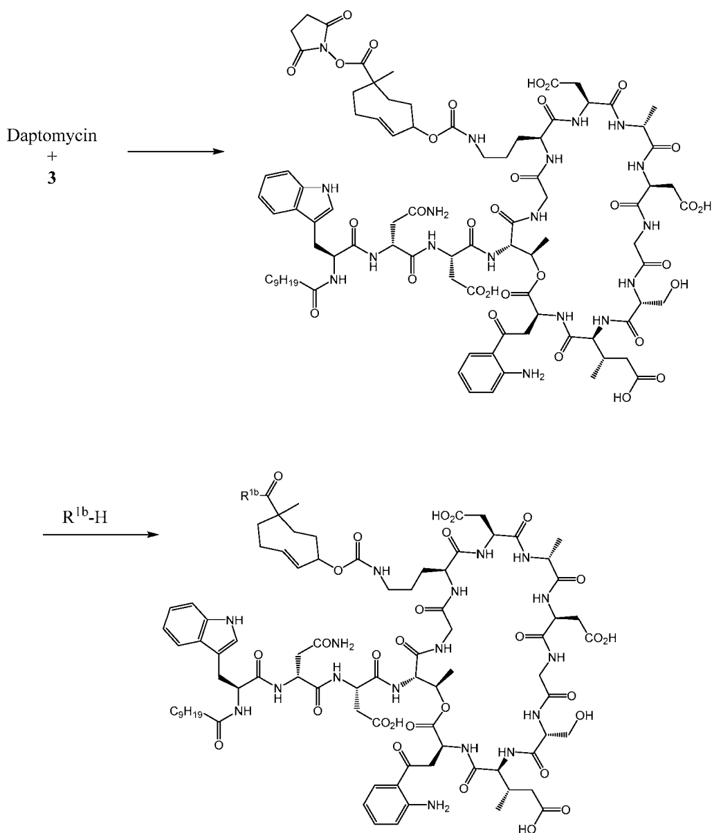
Scheme 3
