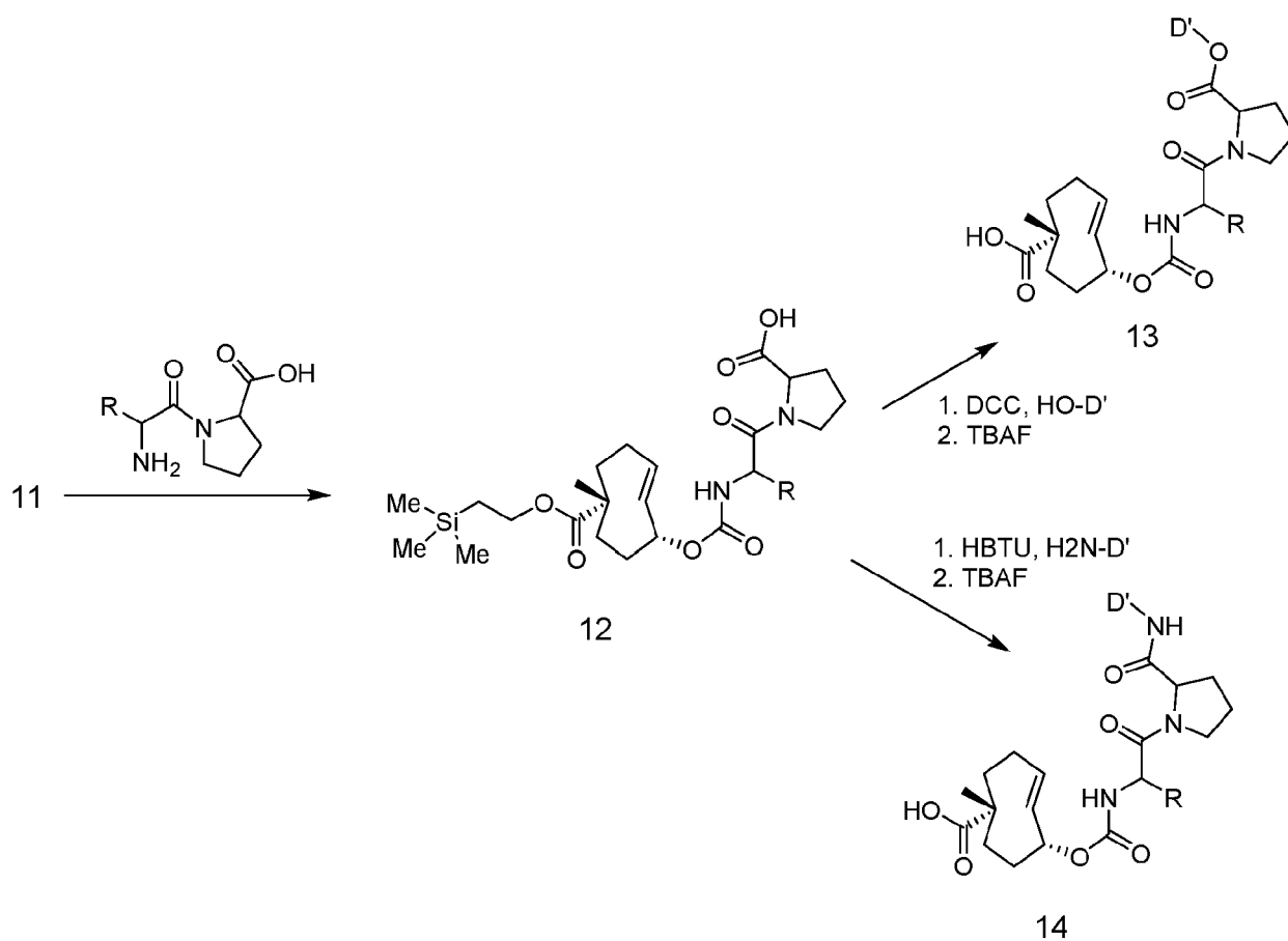
Scheme 5
