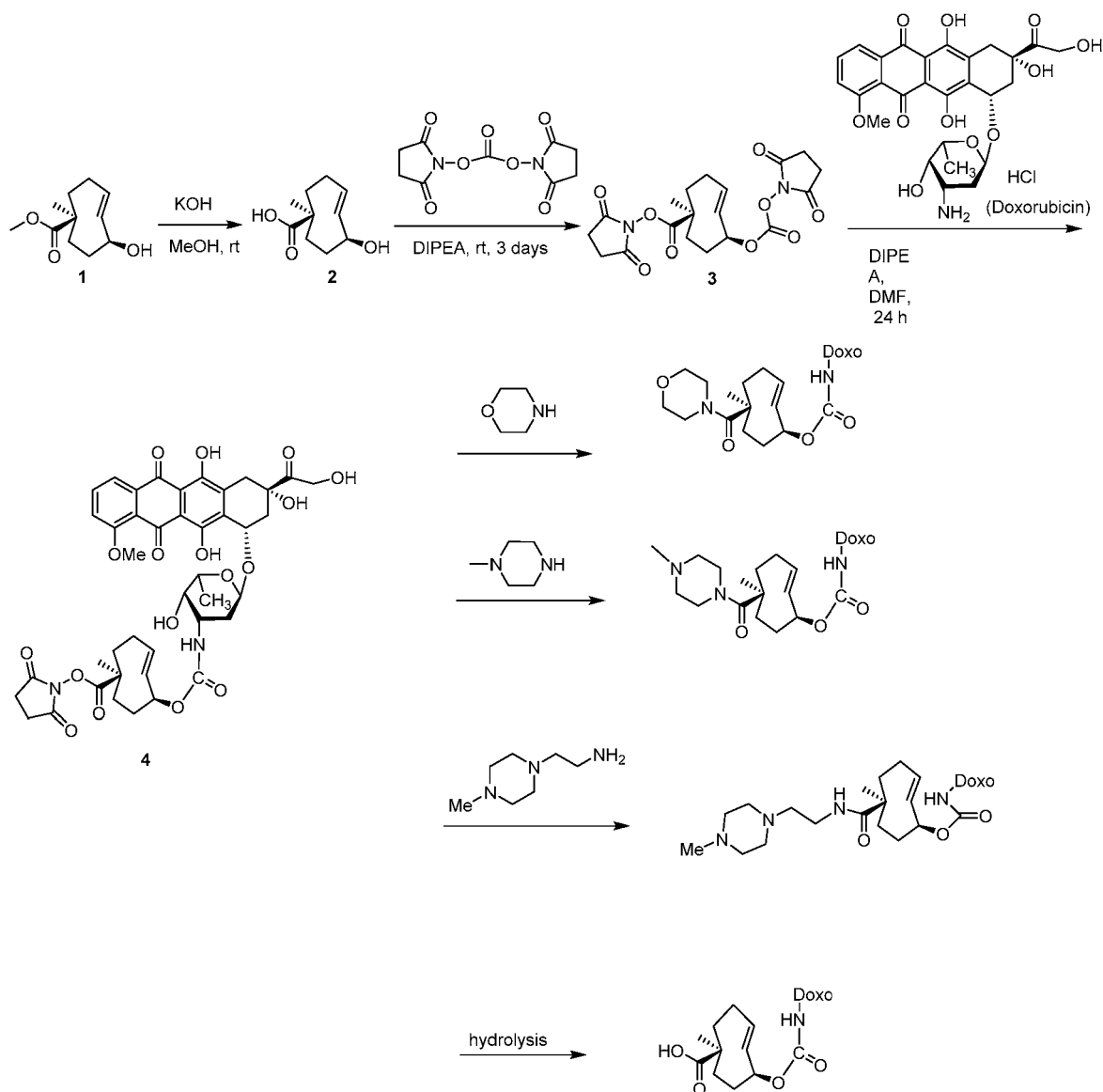
Scheme 2
