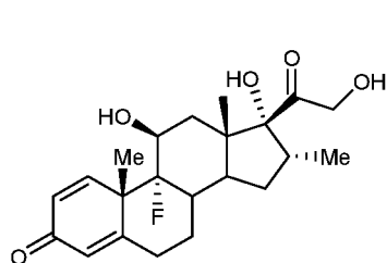
Dexamethasone Corticosteroid
