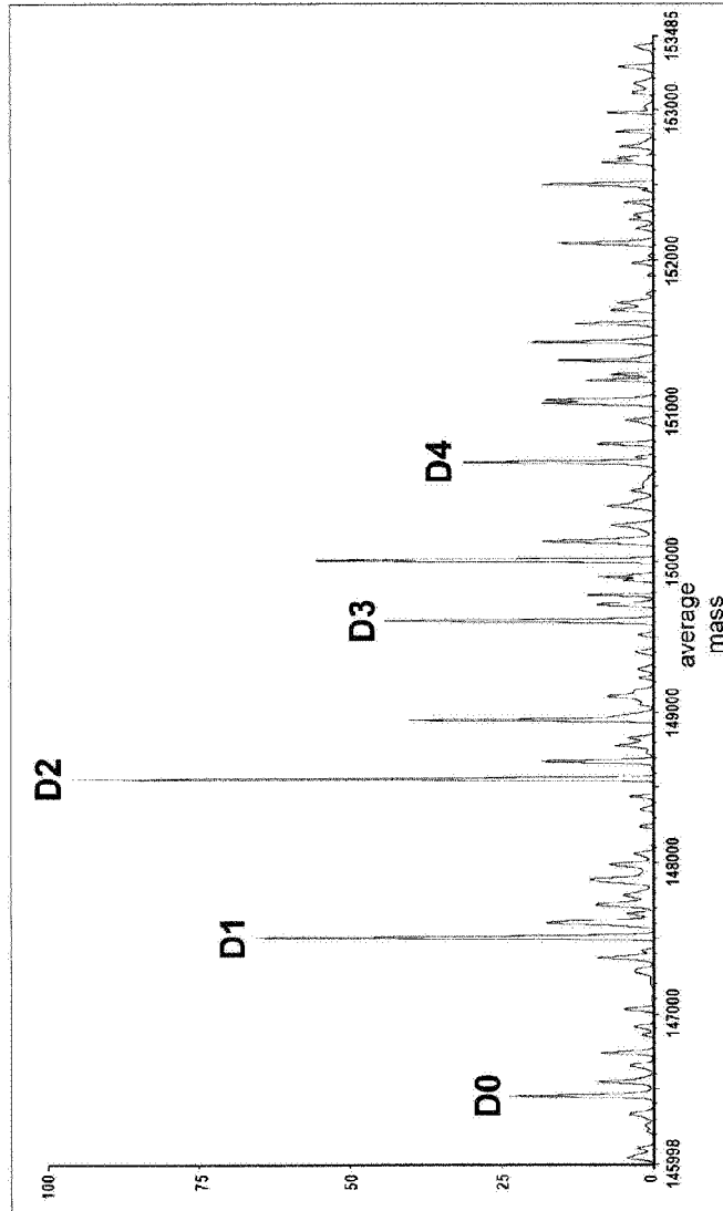
Figure 19: HRMS spectrum of deglycosylated ADC1 at 6 d following a single i.v. administration in non-rodent species at 5 mg/kg (method B2)
