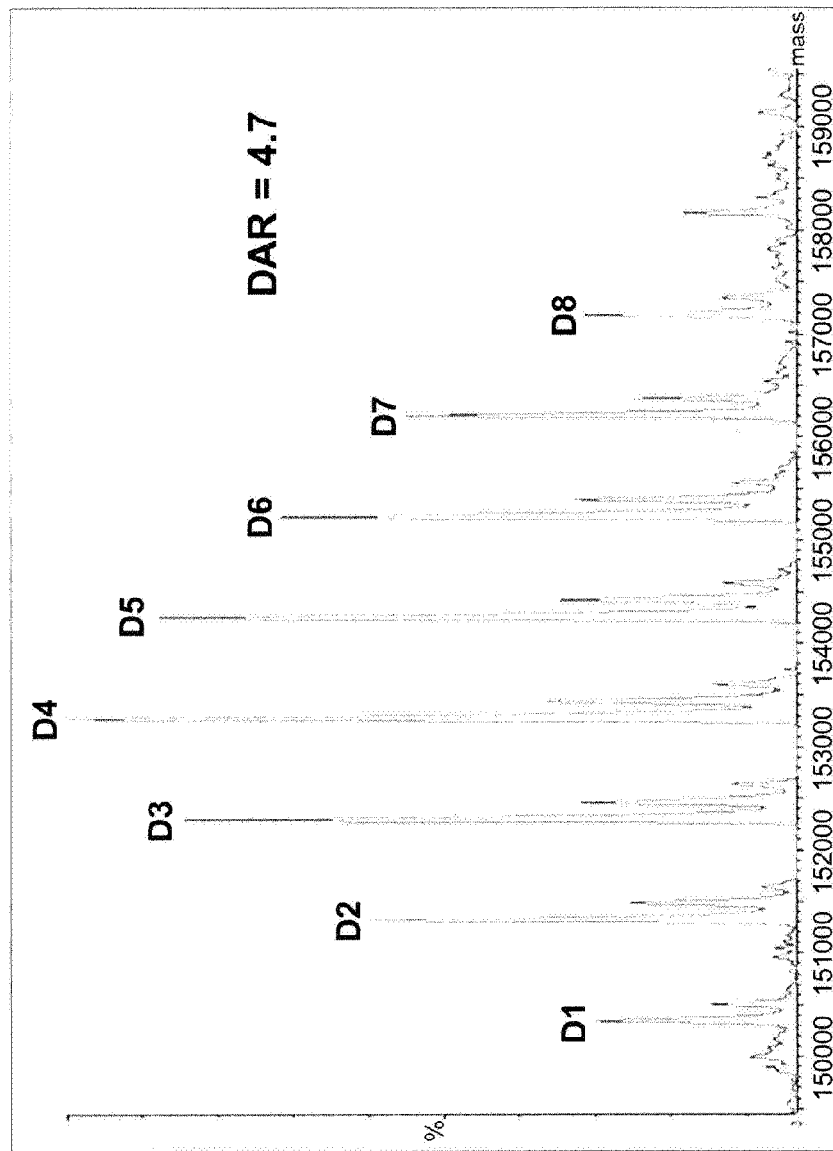
Figure 3: High resolution mass spectrum of Ex.10 (method B1)
