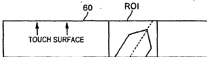
NON-PERPENDICULAR POINTER APPROACHING TOUCH SURFACE CALCULATED CENTER LINE SHOWS EXPECTED POINT OF CONTACT.
