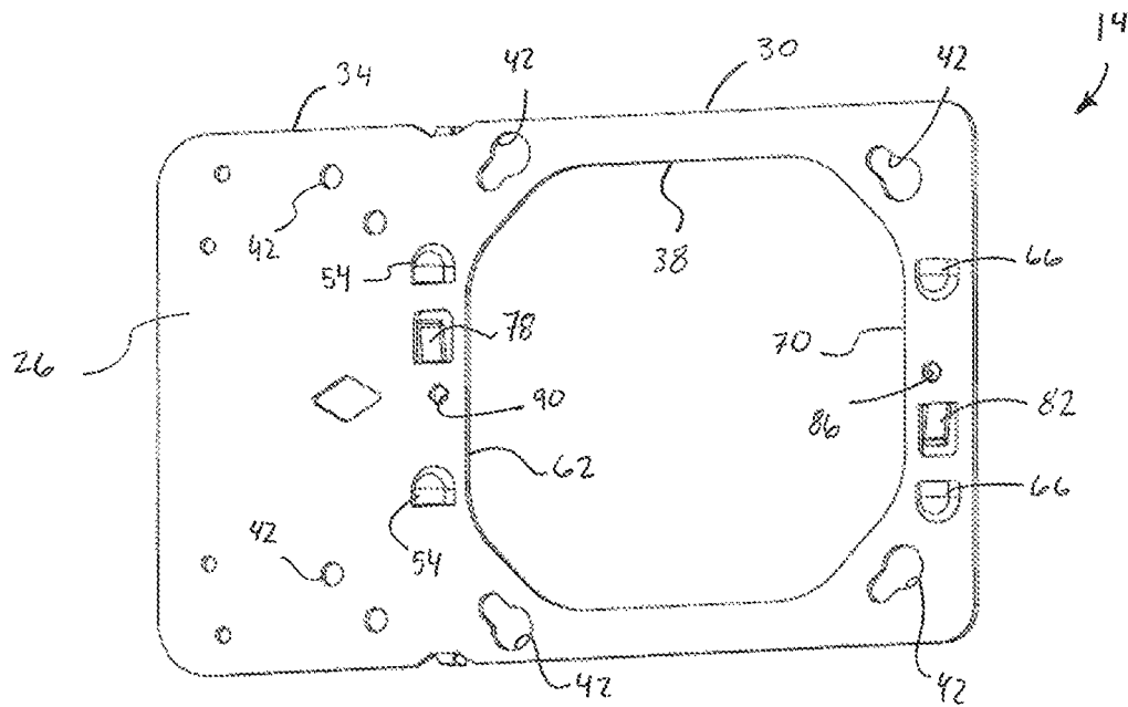
BASE PLATE FIG. 5
