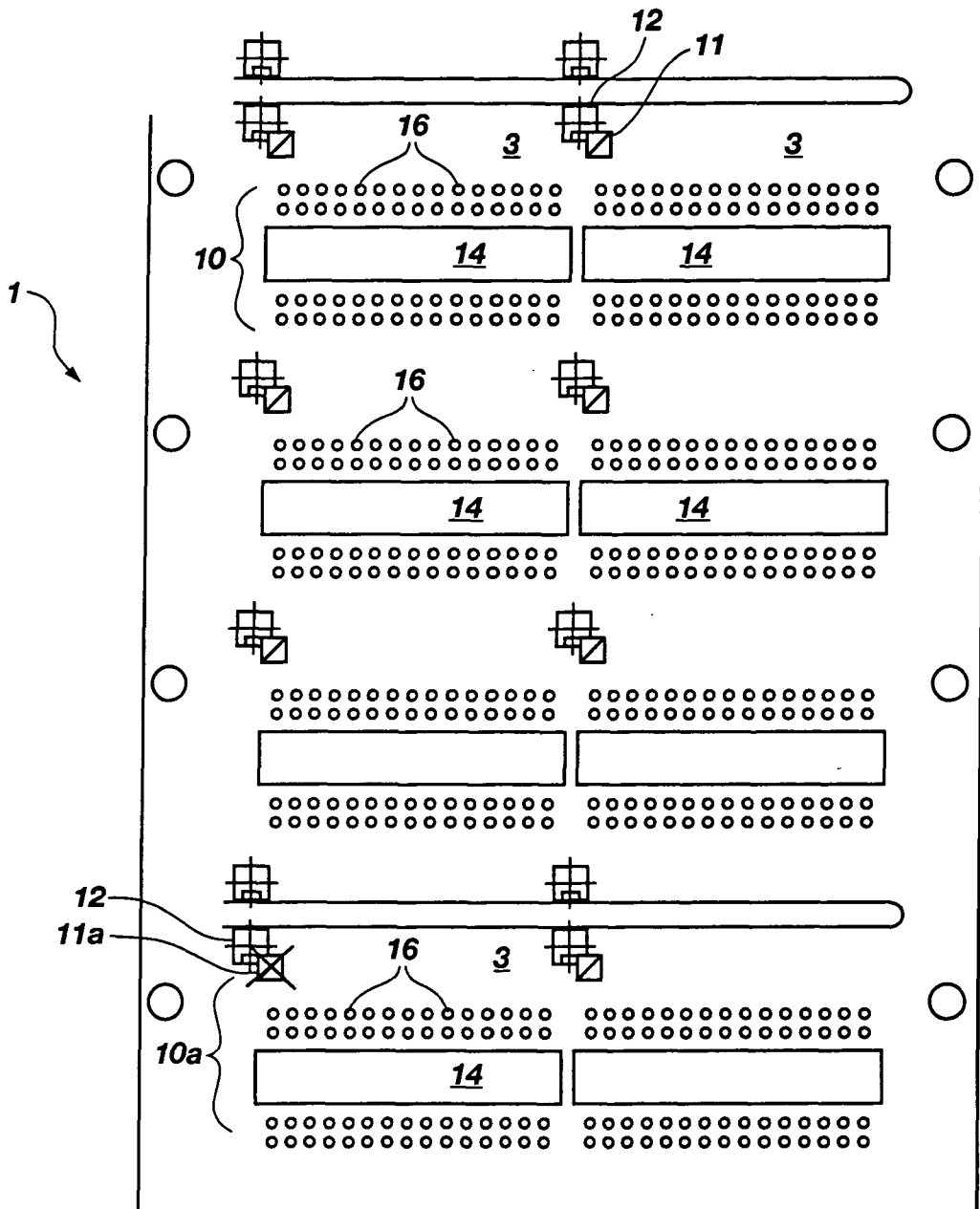
Fig. 2 (PRIOR ART)
