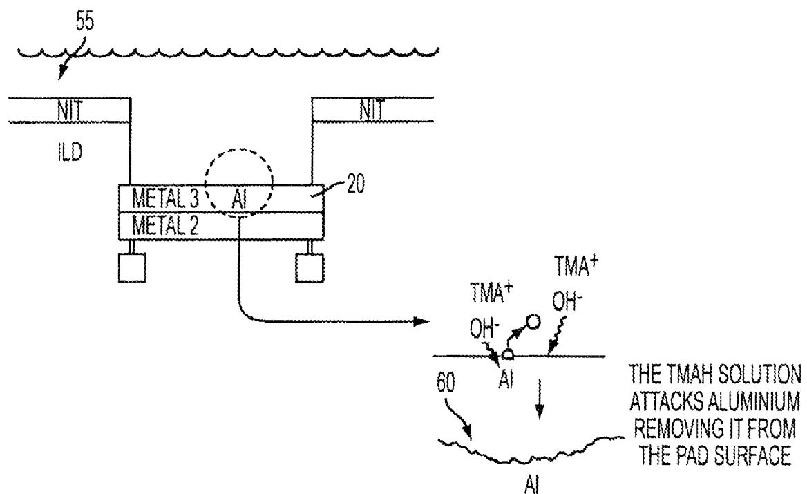
FIG. 2 PRIOR ART
