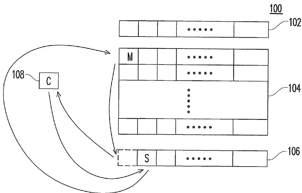
FIG. 1C (PRIOR ART)
