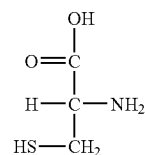
Cysteine
