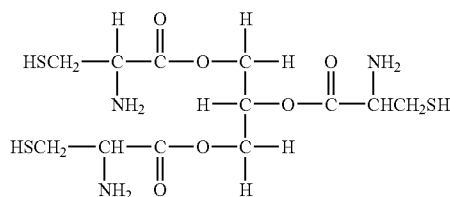
glycerol tricysteinate
