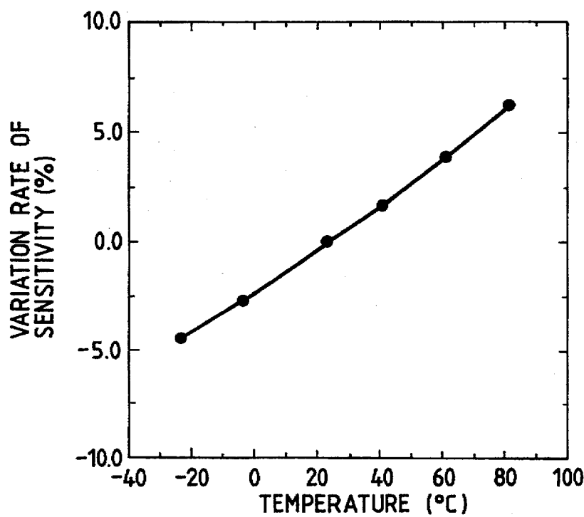
FIG. 5 PRIOR ART
