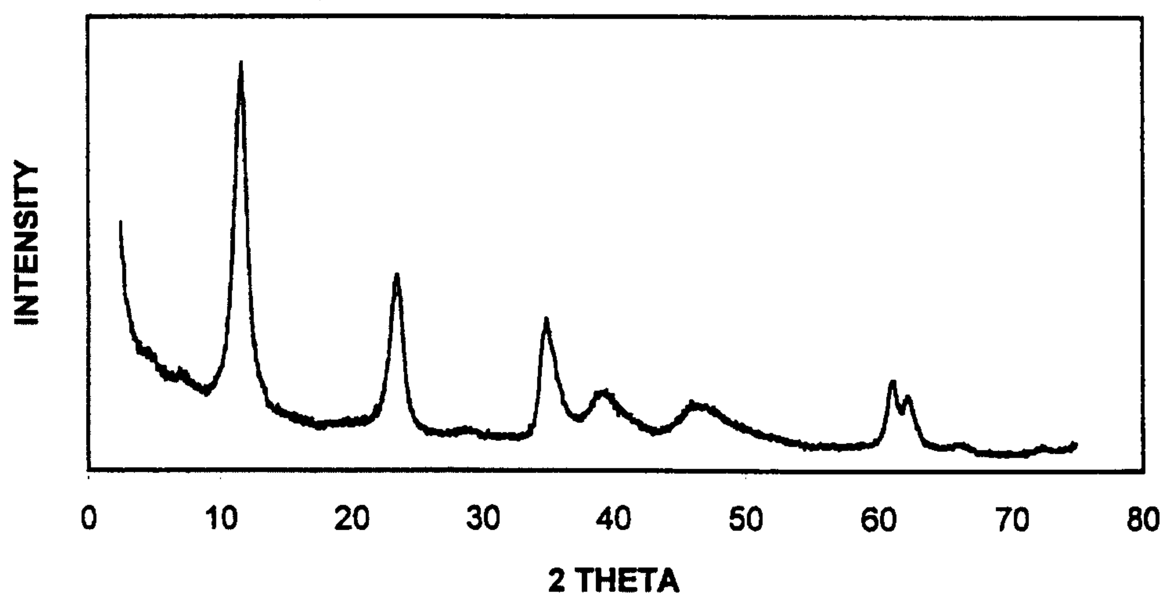
FIGURE 4 Mg-Al acetate anionic clay prepared by coprecipitation
