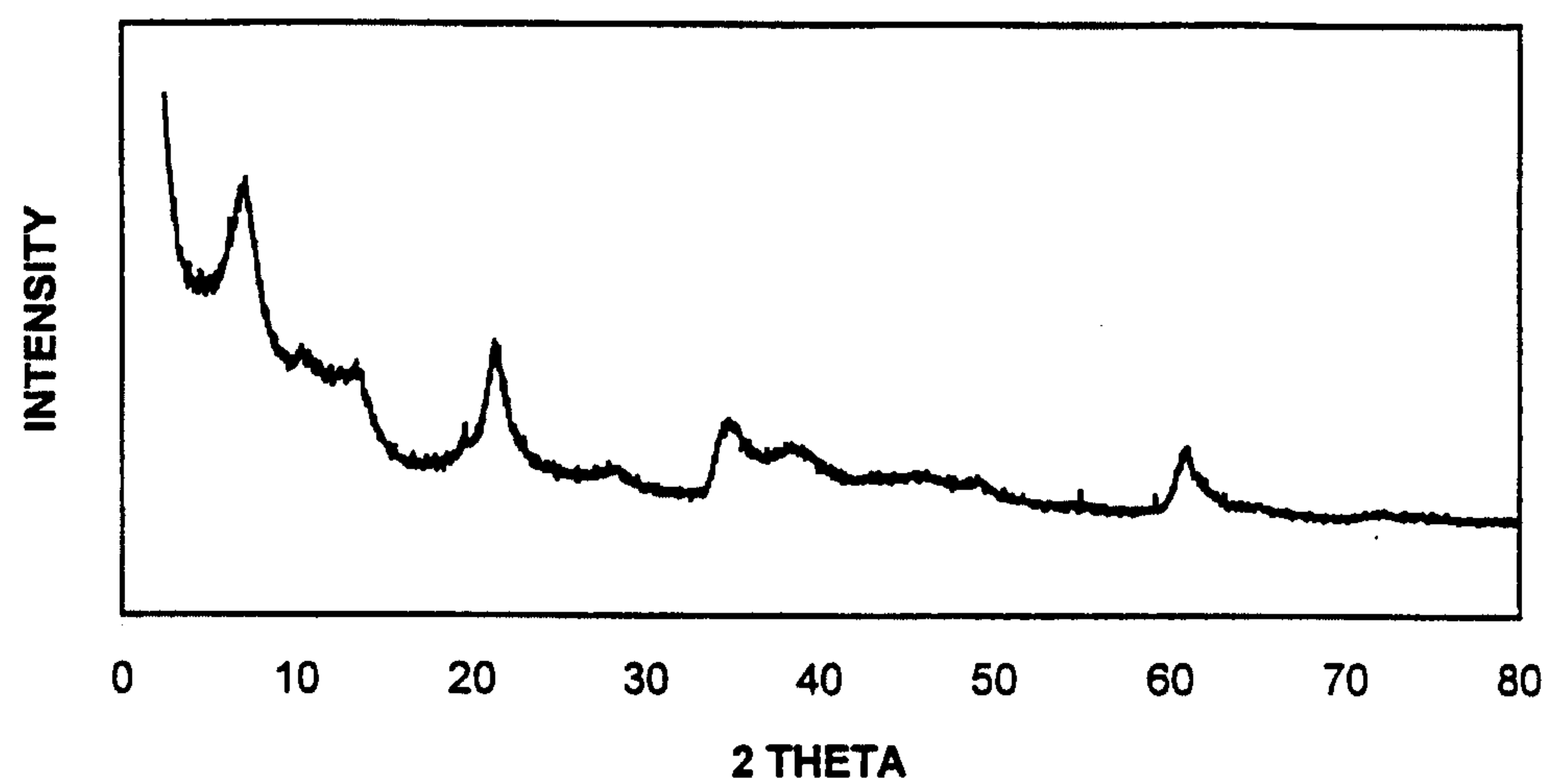
FIGURE 1 commercially available Mg-Al acetate anionic clay
