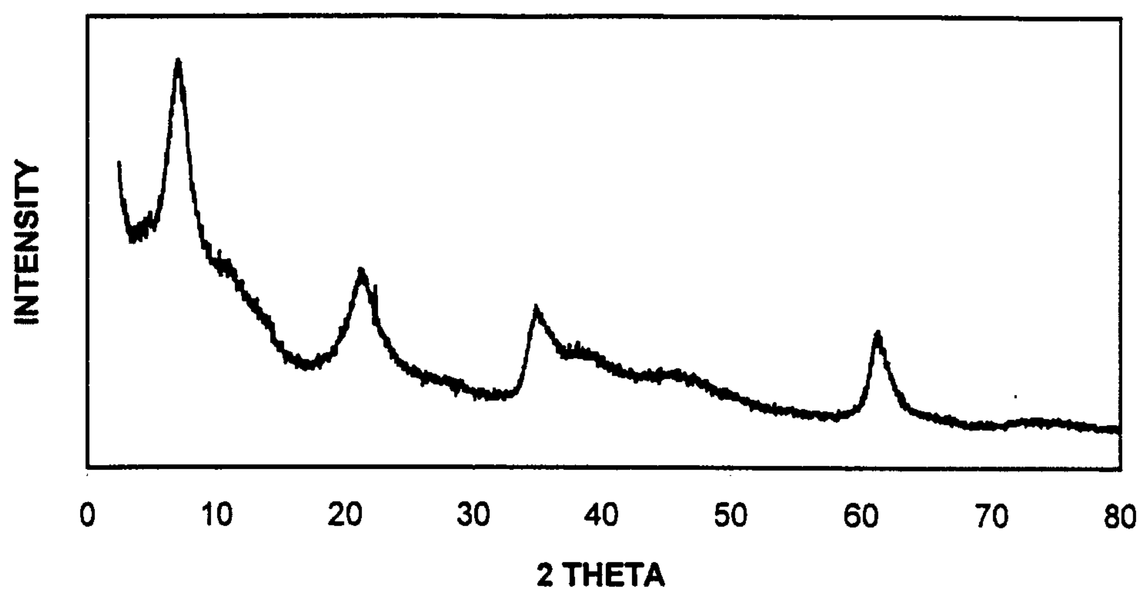
FIGURE 3 Mg-Al acetate anionic clay prepared by coprecipitation
