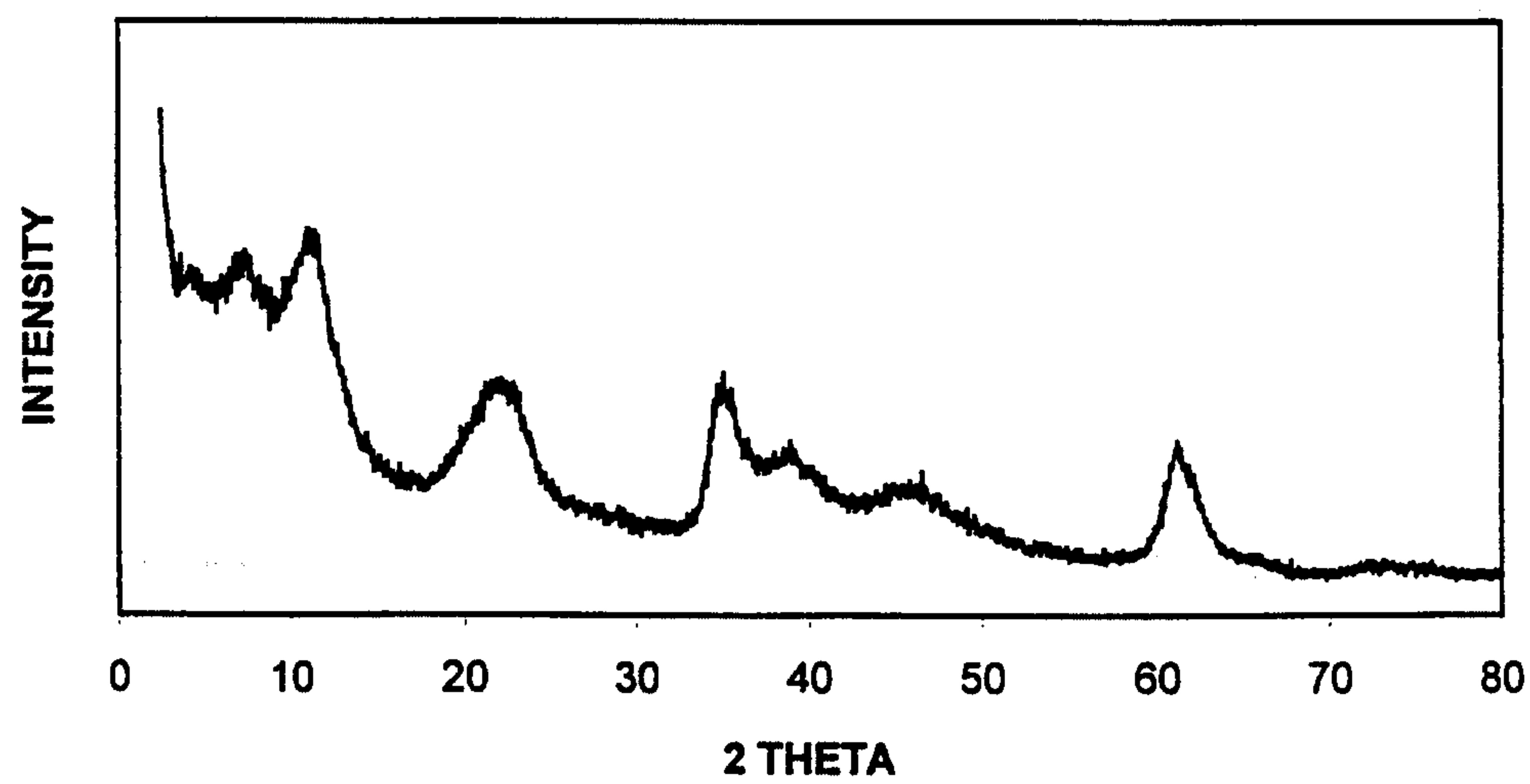
FIGURE 2 Mg-Al acetate anionic clay prepared by coprecipitation
