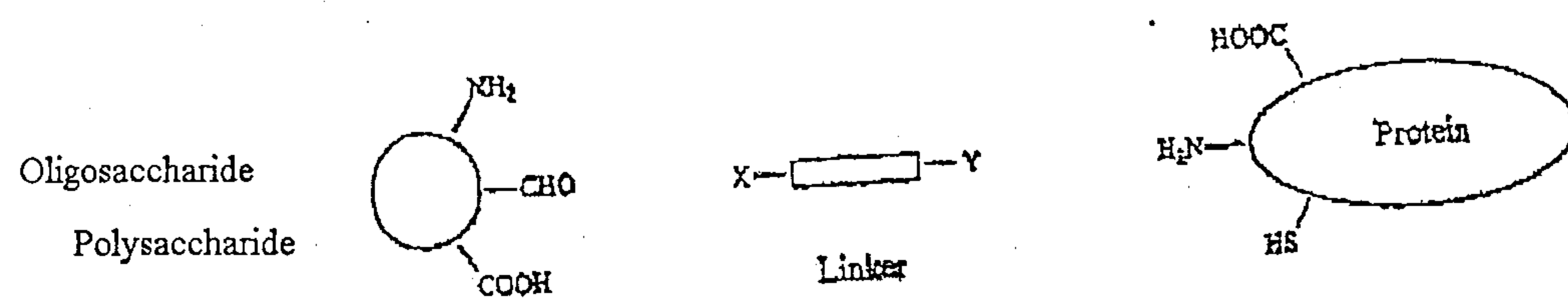
Fig. 1: Neoglycoprotein synthesis
