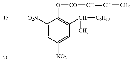
(DINOCAP)
