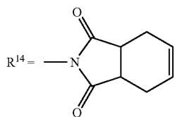
(CAPTAN)
