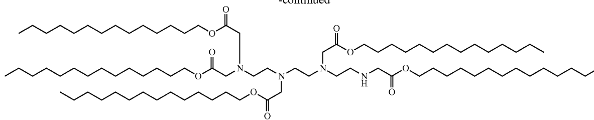
5-tail compound
