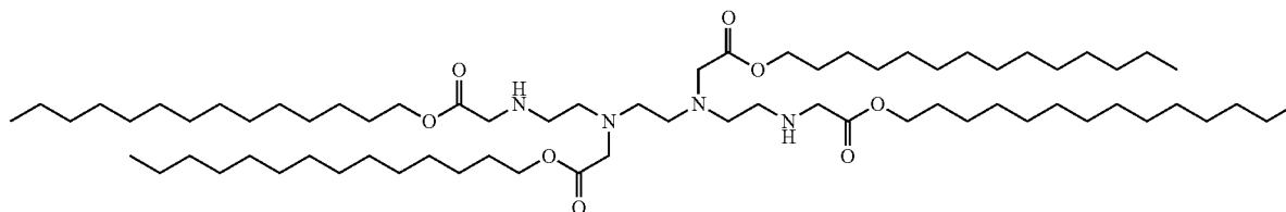
4-tail compound
