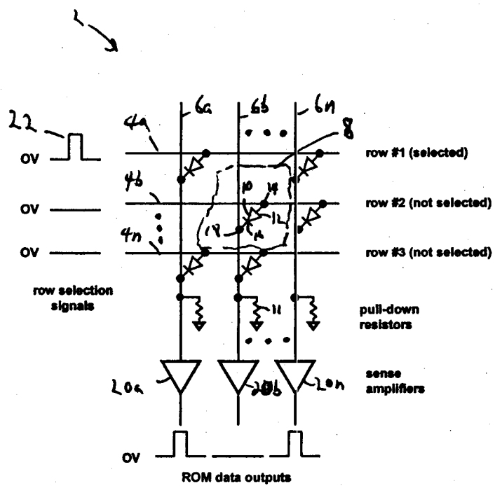
Fig. 1. Prior art. A ROM array using diode elements.
