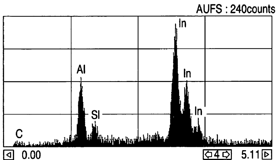
COMPOSITION ANALYSIS PATTERN OF AlInN BY EDX
