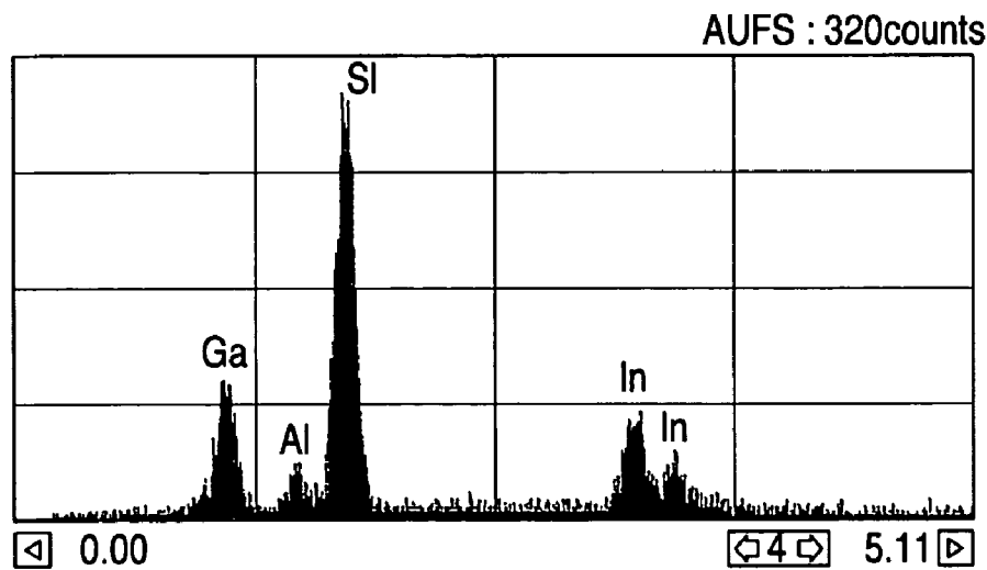
COMPOSITION ANALYSIS PATTERN OF GaAlInN BY EDX
