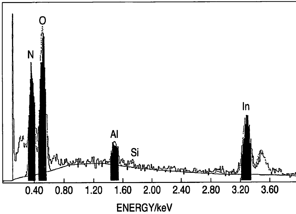
EDX SPECTRUM OF OXINITRIDE MATERIAL
