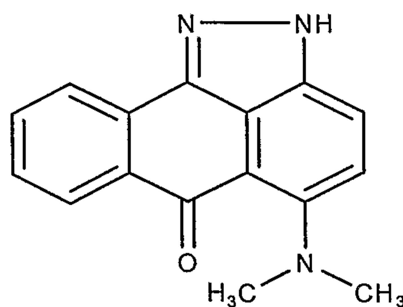
5-Dimethylamino-2H- dibenzo[cd,g]indazol-6-one;
