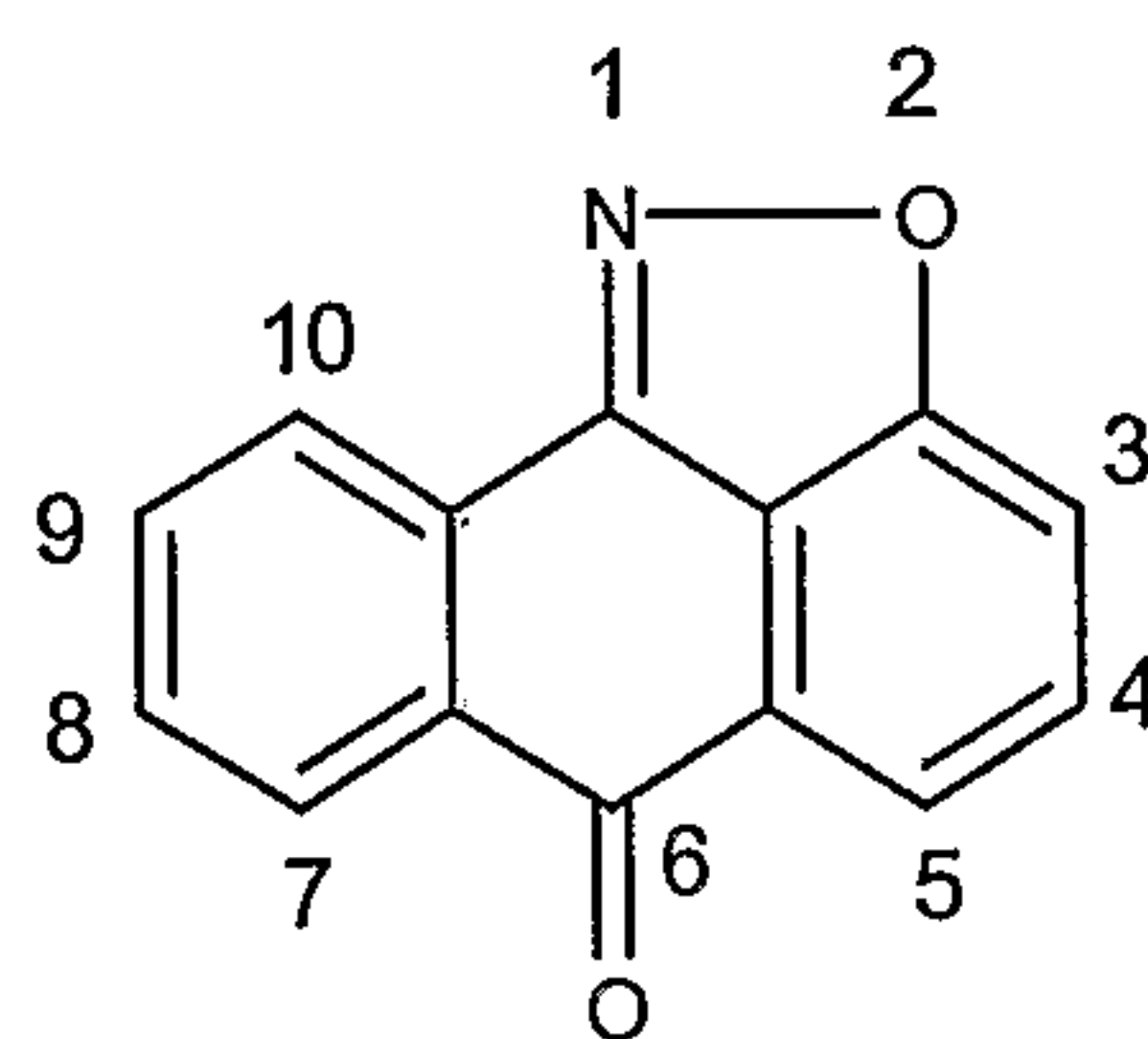
2-Oxa-1-aza-aceanthrylen-6-one (IIIC)
