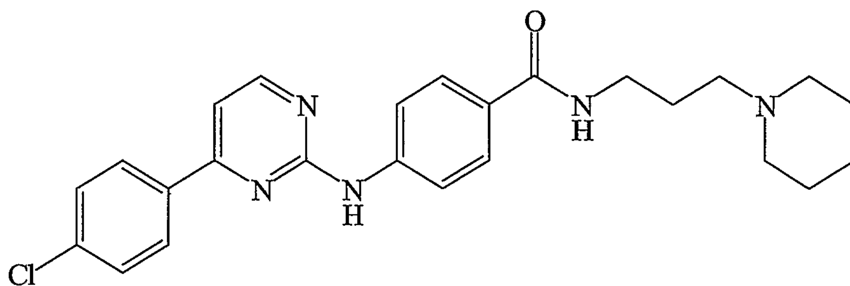
4-[4-(4-Chloro-phenyl)-pyrimidin-2-ylamino]- N -(3-piperidin-1-yl-propyl)-benzamide ;
