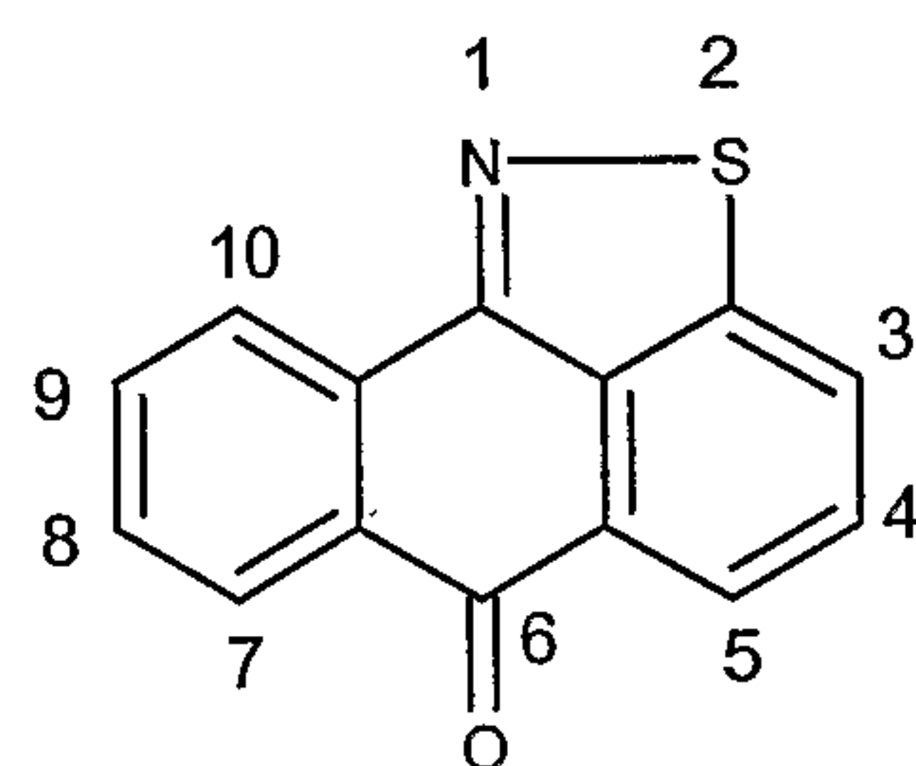
Anthra[9,1- cd ]isothiazol-6-one (IIIE)
