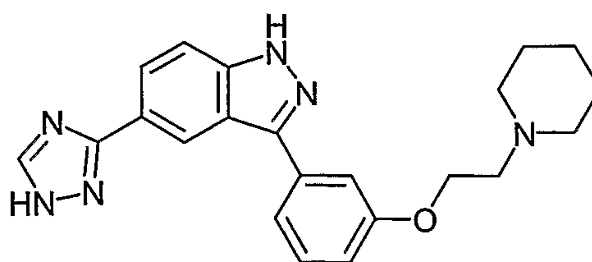
3-[3-(2-Piperidin-1-yl-ethoxy)-phenyl]-5-(1H-[1,2,4]triazol-3-yl)-1H-indazole ;
