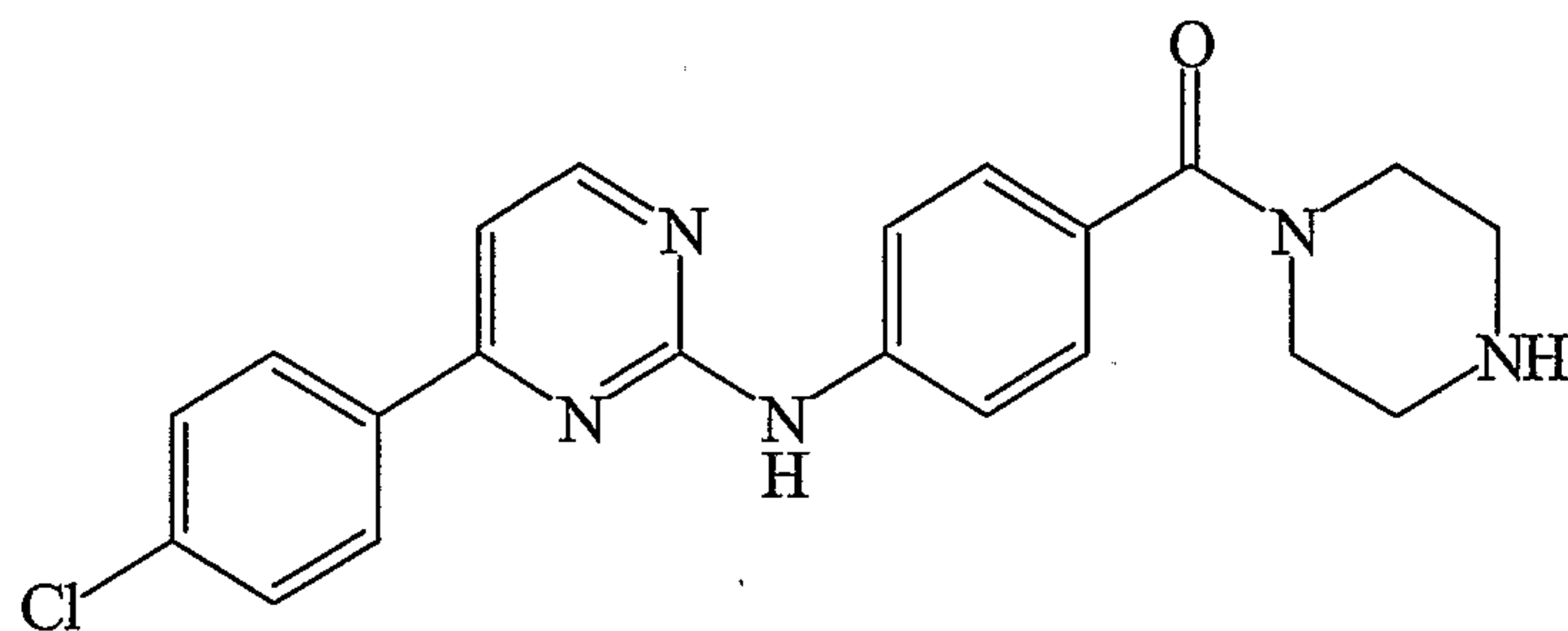
{4-[4-(4-Chloro-phenyl)-pyrimidin-2-ylamino]-phenyl}-piperazin-1-yl-methanone ;
