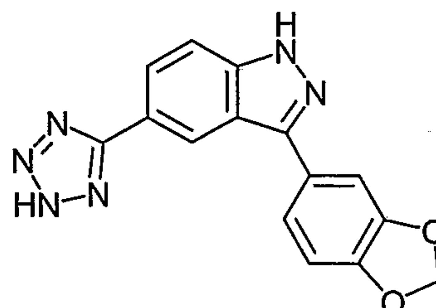
3-Benzo[1,3]dioxol-5-yl-5-(2 H -tetrazol-5-yl)-1 H -indazole ;
