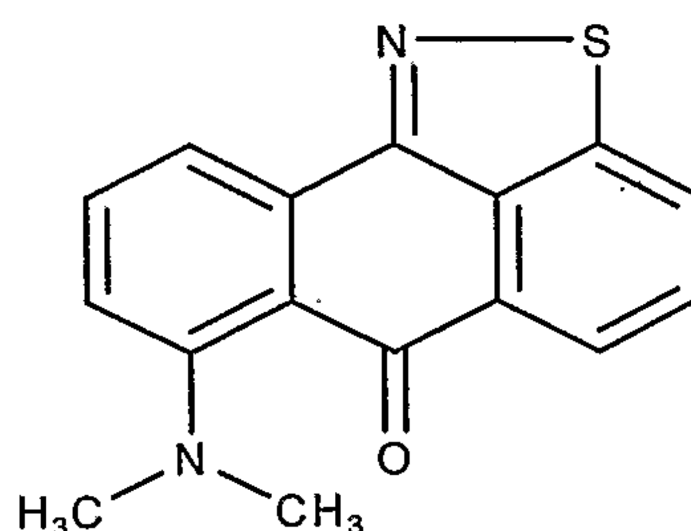
7-Dimethylamino-anthra[9,1- cd ]isothiazol-6-one ;
