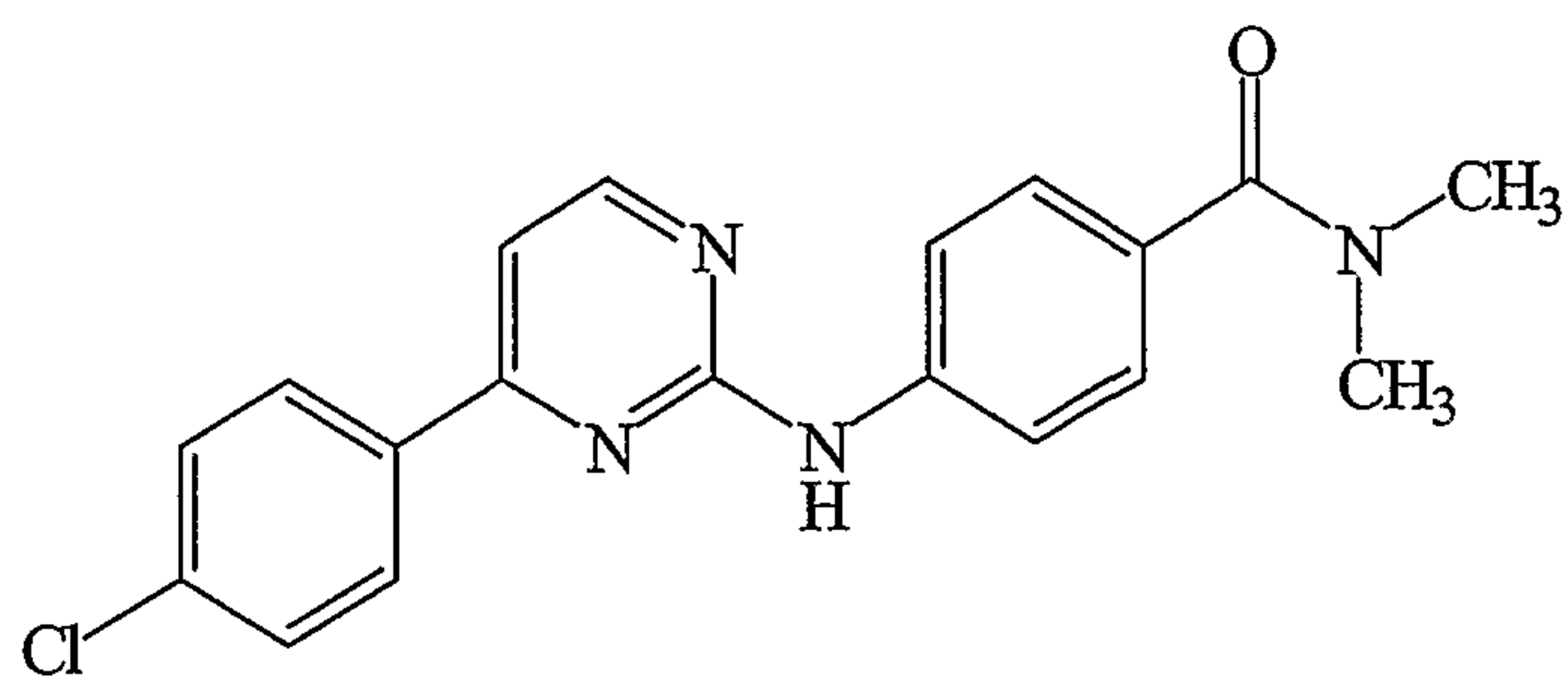
4-[4-(4-Chloro-phenyl)-pyrimidin-2-ylamino]- N,N -dimethyl-benzamide ;
