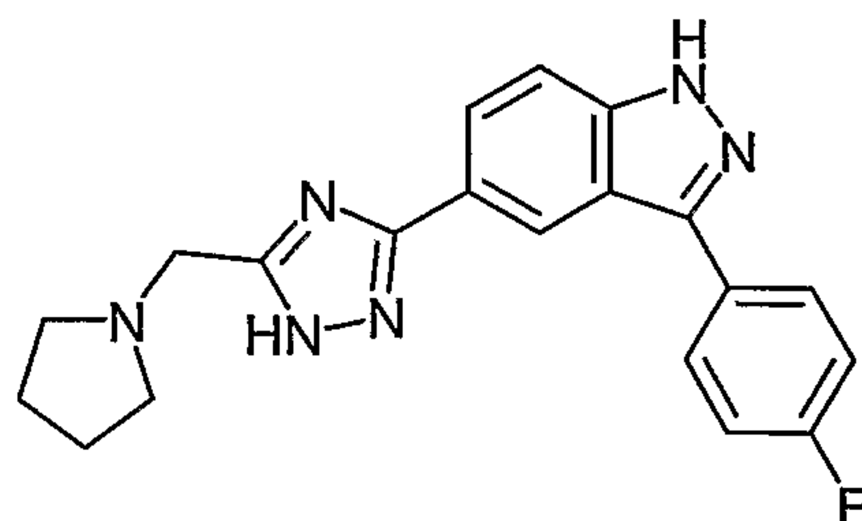
3-(4-Fluoro-phenyl)-5-(5-pyrrolidin-1-ylmethyl-1 H -[1,2,4]triazol-3-yl)-1 H -indazole ;
