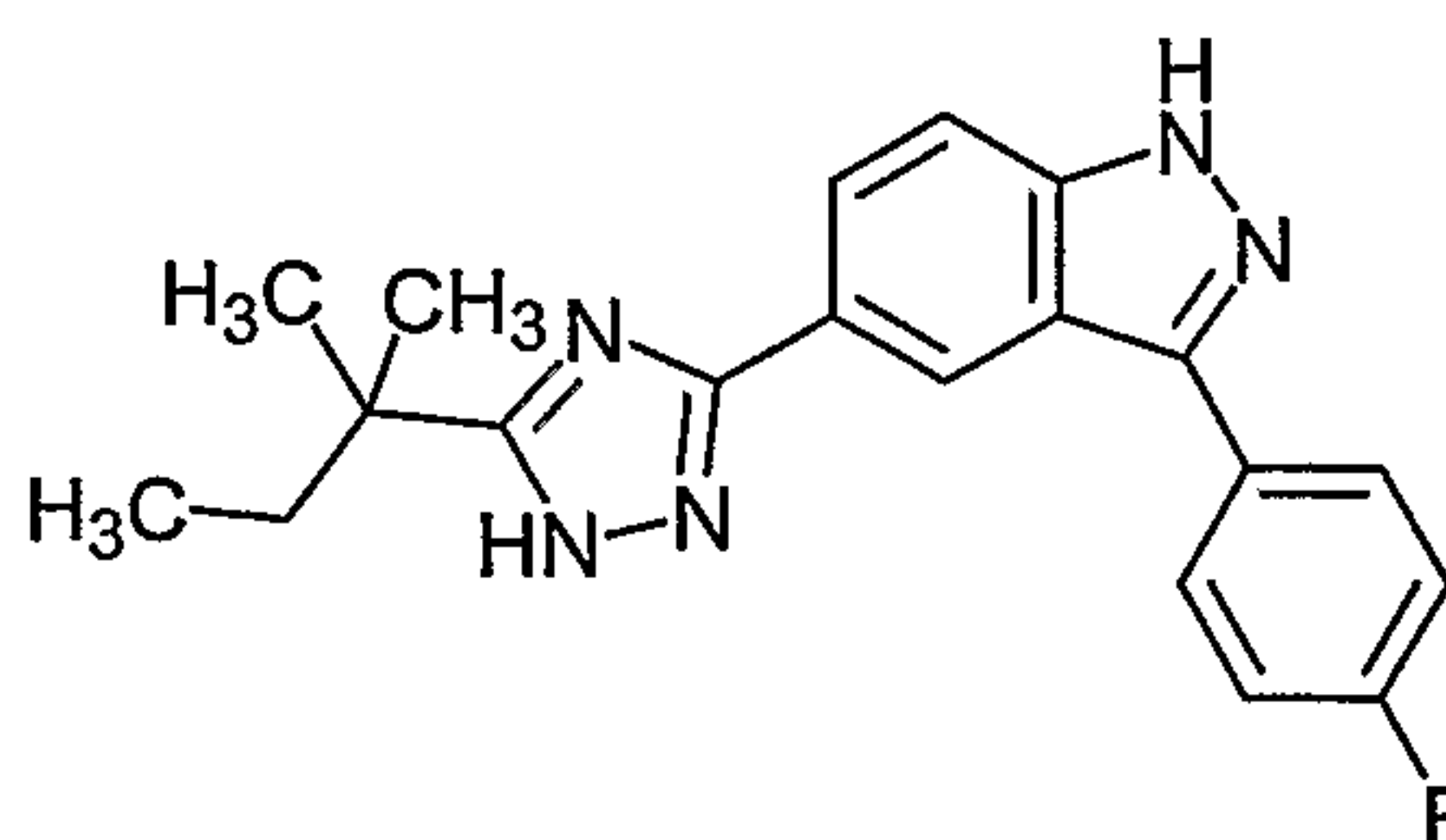
5-[5-(1,1-Dimethyl-propyl)-1 H -[1,2,4]triazol-3-yl]-3-(4-fluoro-phenyl)-1 H -indazole ;
