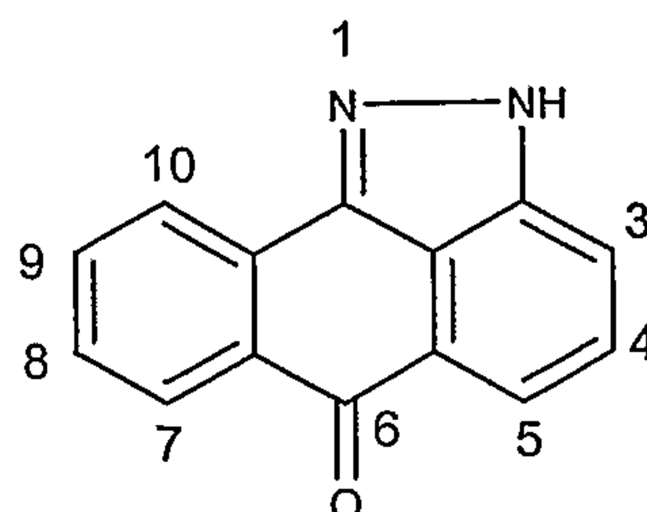
2H-Dibenzo[cd,g]indazol-6-one (IIIF)
