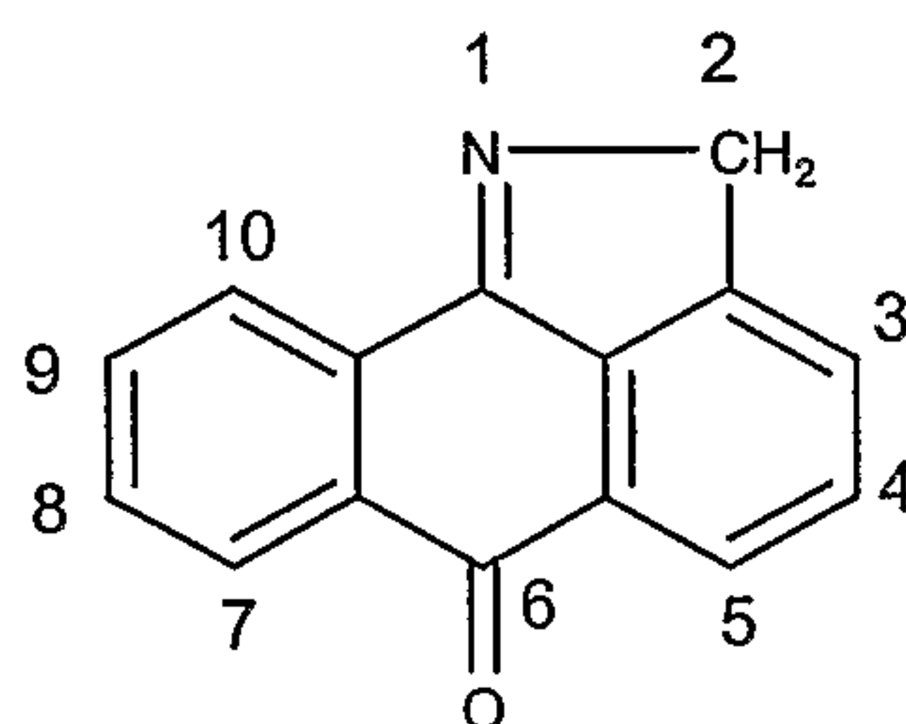
2H-Dibenzo[cd,g]indol-6-one (IIIA)
