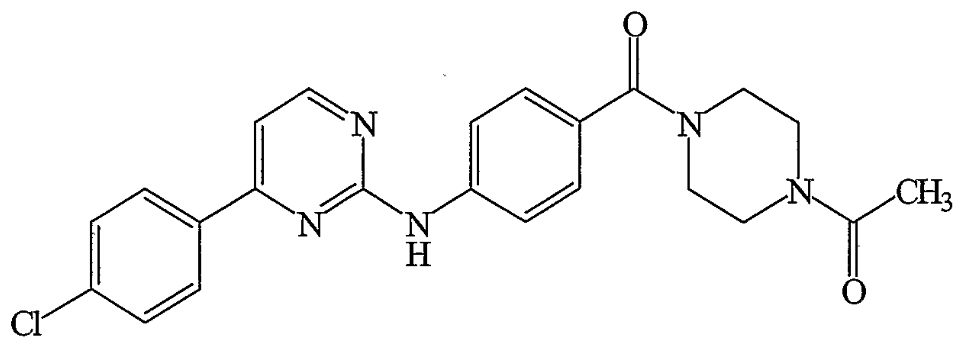
1-(4-{4-[4-(4-Chloro-phenyl)-pyrimidin-2-ylamino]-benzoyl}-piperazin-1-yl)-ethanone ;
