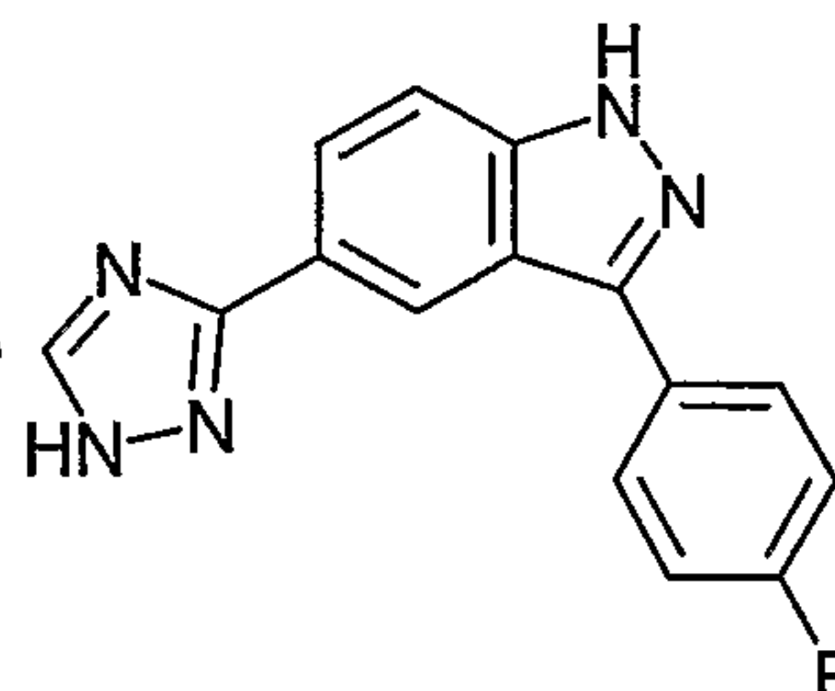
3-(4-Fluoro-phenyl)-5-(1H-[1,2,4]triazol-3-yl)-1H-indazole;
