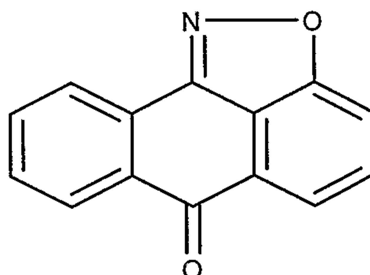
2-Oxa-1-aza-aceanthrylen-6-one;
