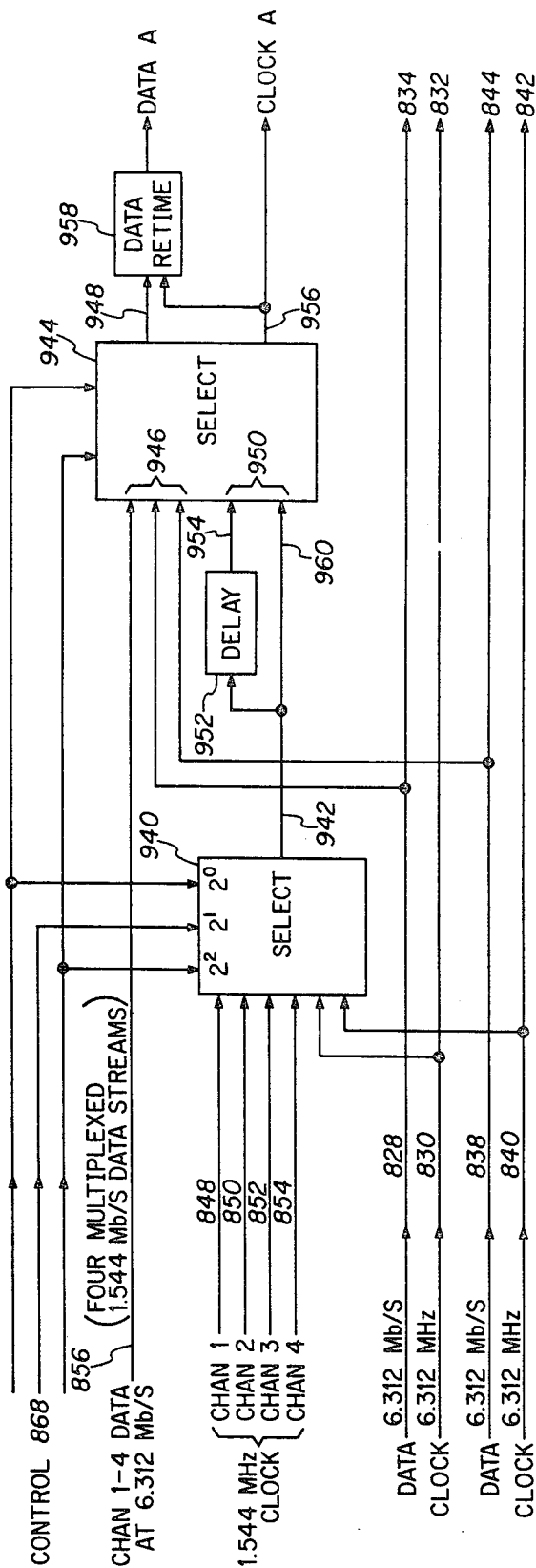
FIG. 15 SECTION A OF DATA COMPARATOR INTERFACE
