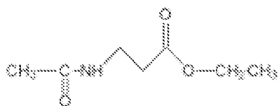
N-Acetyl Beta Alanine Ethyl Ester
