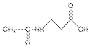
N-acetyl beta alanine
