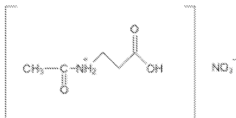
N-Acetyl Beta Alanine Nitrate
