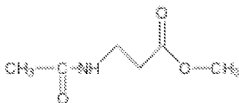
N-acetyl Beta Alanine Methyl Ester
