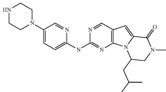
Compound 47
