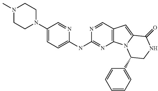
Compound 22
