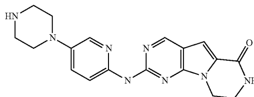
Compound 3
