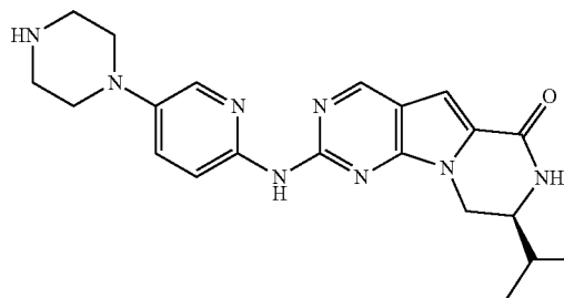
Compound 24
