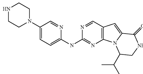
Compound 8
