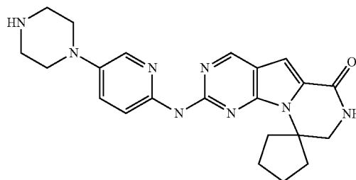
Compound 30
