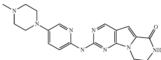
Compound 1
