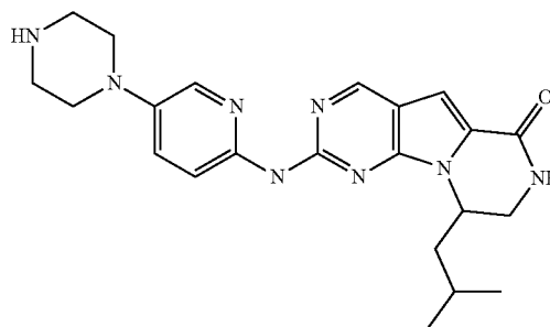
Compound 46
