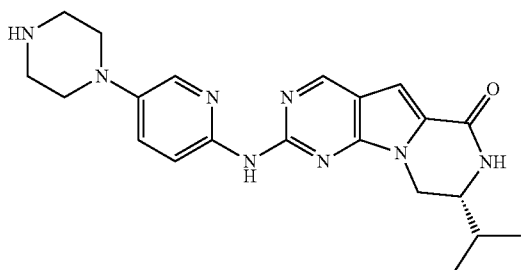
Compound 25
