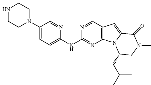
Compound 15
