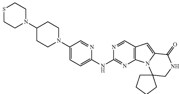
Compound 43
