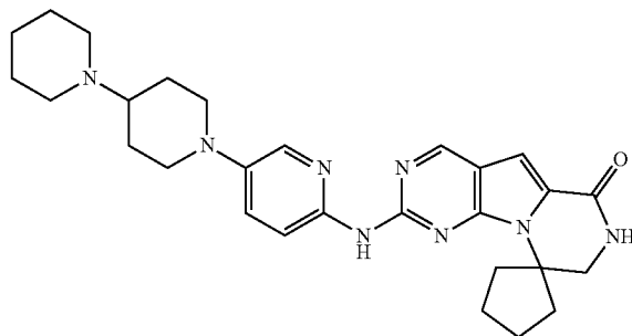
Compound 40
