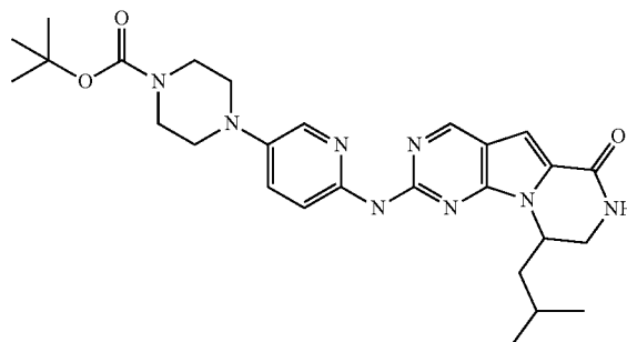
Compound 50
