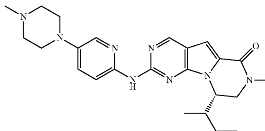
Compound 18
