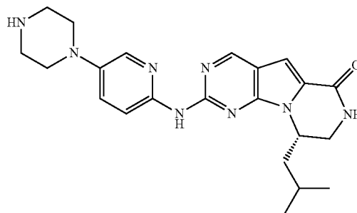
Compound 13
