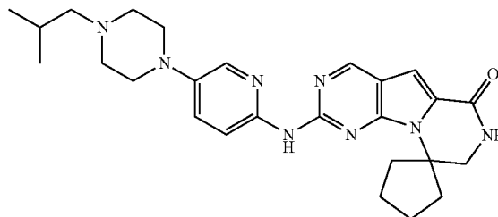
Compound 36
