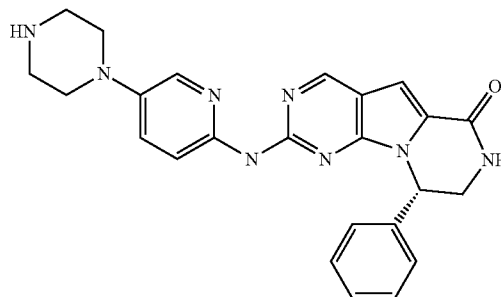
Compound 23
