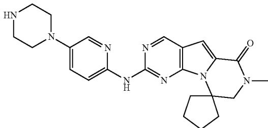
Compound 31
