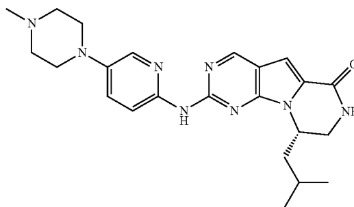
Compound 12
