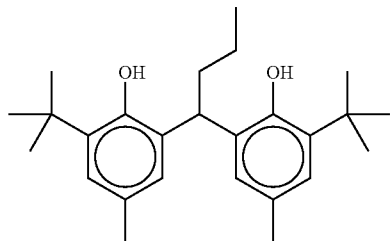
Reducing Agent Complex-1
