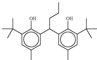
Hydrogen Bond-Forming Compound-1
