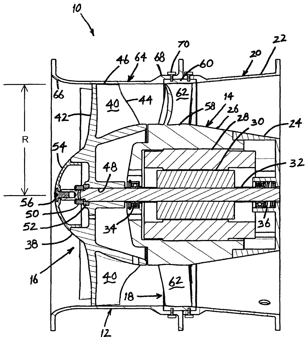
Fig. 1 (Prior Art)
