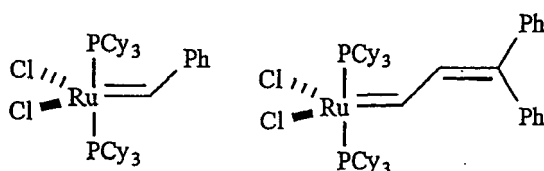
Grubbs Catalyst 1
