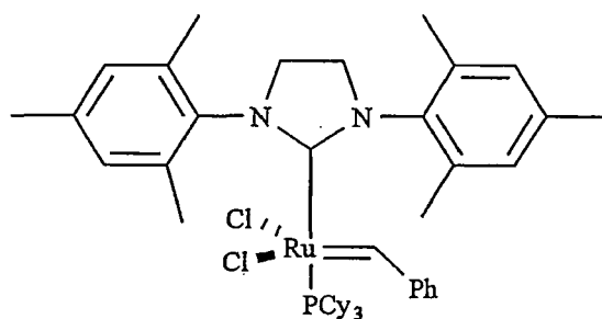
Grubbs Catalyst 3
