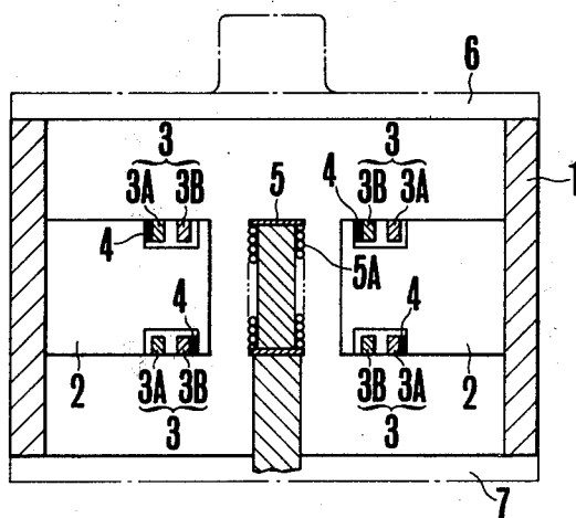
FIG.2 (PRIOR ART)
