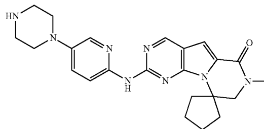
Compound 31
