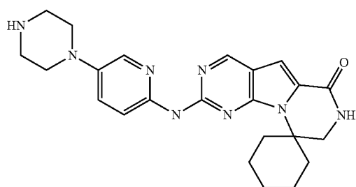
Compound 28
