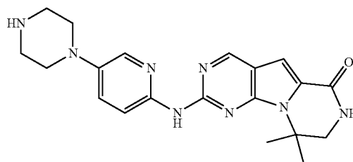
Compound 26
