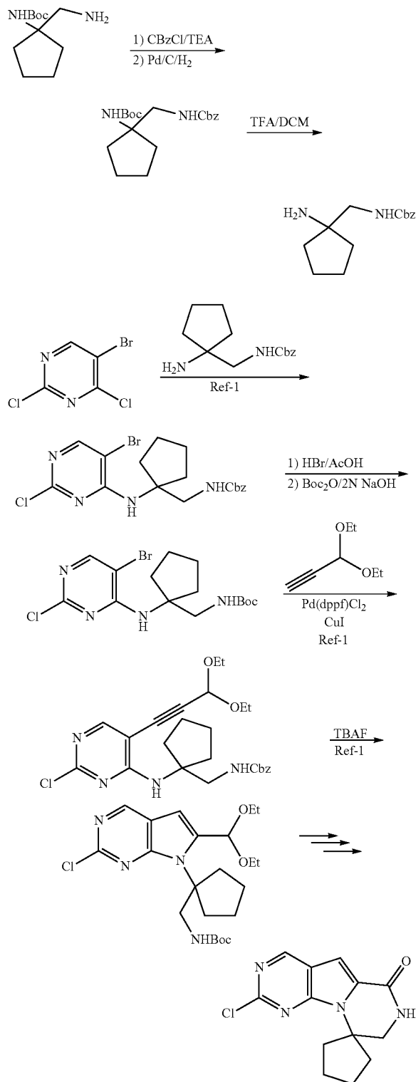
Scheme 3
