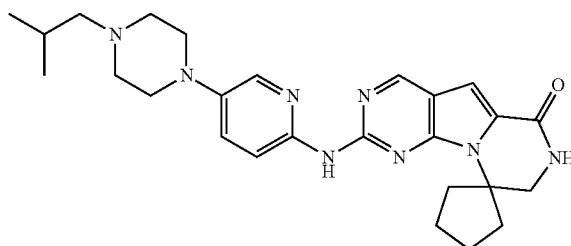
Compound 36
