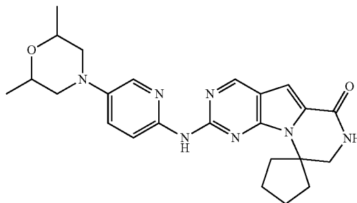
Compound 37
