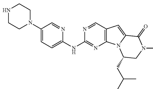
Compound 15
