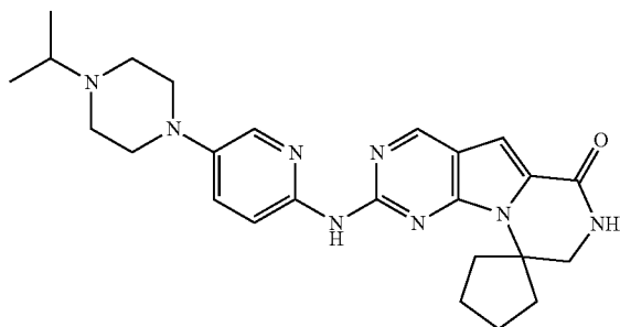
Compound 35
