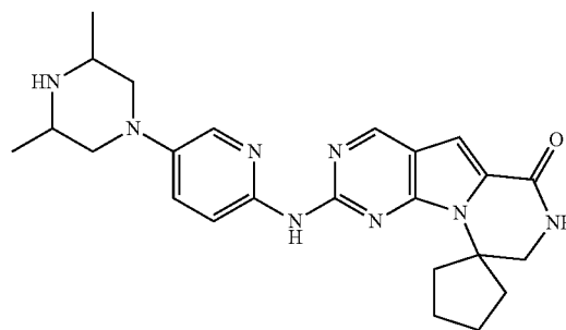
Compound 42
