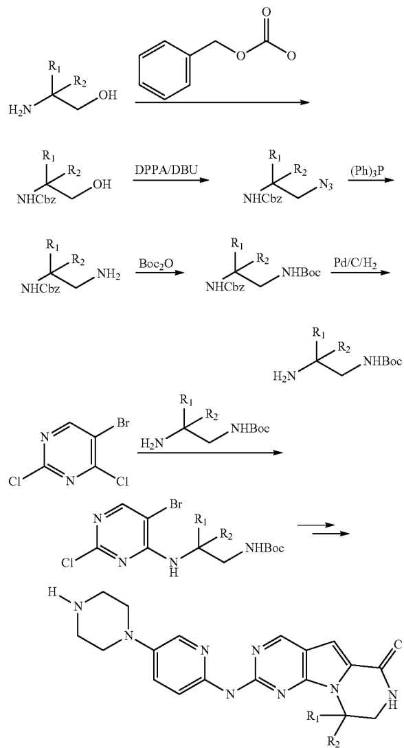
Scheme 4
