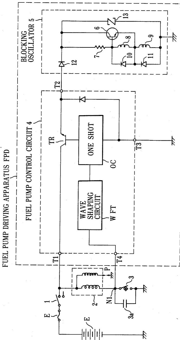
FIG. 1 (PRIOR ART)
