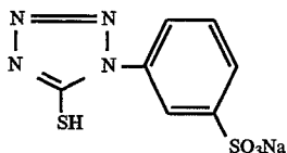
Compound (N)
