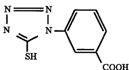
Compound (N)
