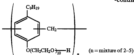
Compound (S-1)
