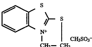
Compound (I)
