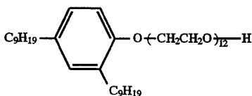
Compound (J)
