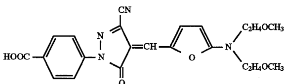
Compound (O)
