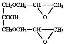
Compound i
