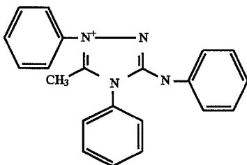
Compound (H)
