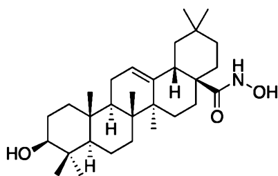
(3β) 3-Hydroxy-N-hydroxy-olean-12-en-28-amide
