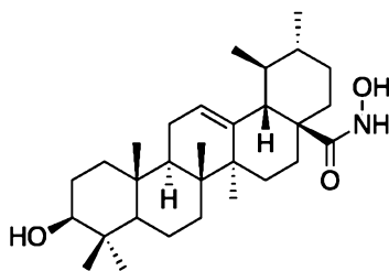
(3β) 3-Hydroxy-N-hydroxy-urs-12-en-28-amide
