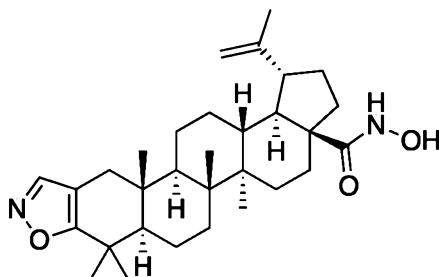
Lup-2-eno[2,3-d]isoxazol- N -hydroxy-28-amide
