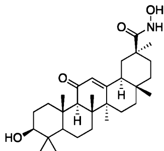
(3 \beta ) 3-Hydroxy-11-oxo-olean-12-en-N-hydroxy-29-amide
