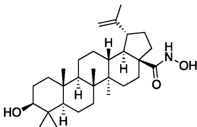
(3β) 3-Hydroxy-N-hydroxy-lup-20(29)-en-28-amide
