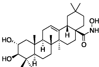
(2α,3β) 2,3-Dihydroxy-N-hydroxy-olean-12-en-28-amide
