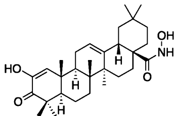
2-Hydroxy-3-oxo-oleana-1,12-dien- N -hydroxy-28-amide
