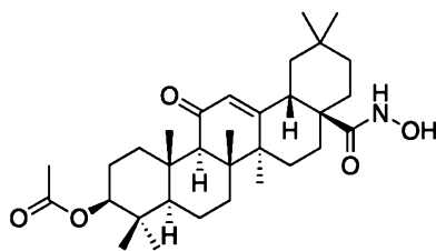
(3β) 3-Acetyloxy-11-oxo-olean-12-en-N-hydroxy-28-amide
