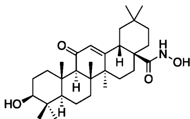
(3β) 3-Hydroxy-11-oxo-olean-12-en-N-hydroxy-28-amide
