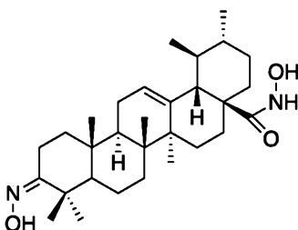
3-Hydroxyimino-N-hydroxy-urs-12-en-28-amide
