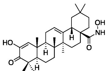
2-Hydroxy-3-oxo-oleana-1,12-dien-N-hydroxy-28-amide
