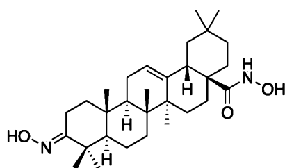
3-Hydroxyimino-N-hydroxy-olean-12-en-28-amide
