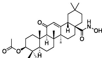
(3 \beta ) 3-Acetyloxy-11-oxo-olean-12-en- N -hydroxy-28-amide
