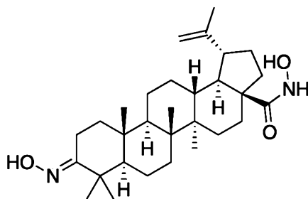
3-Hydroxyimino-N-hydroxy-lup-20(29)-en-28-amide
