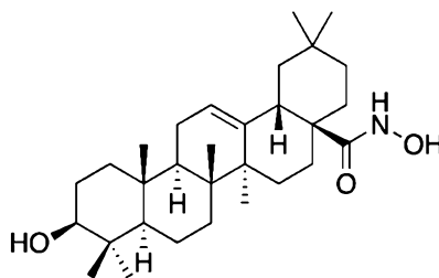
(3β) 3-Hydroxy- N -hydroxy-olean-12-en-28-amide
