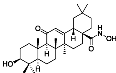
(3β) 3-Hydroxy-11-oxo-olean-12-en- N -hydroxy-28-amide
