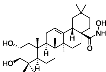
(2α,3β) 2,3-Dihydroxy- N -hydroxy-olean-12-en-28-amide
