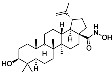
(3 \beta ) 3-Hydroxy- N -hydroxy-lup-20(29)-en-28-amide
