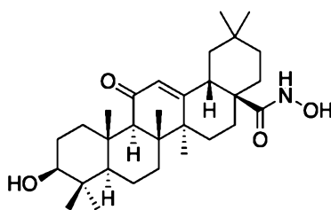
(3 \beta ) 3-Hydroxy-11-oxo-olean-12-en- N -hydroxy-28-amide
