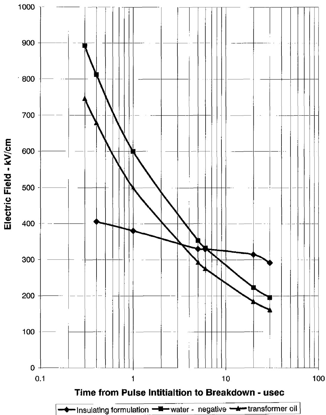
Dielectric Strength vs. Delay To Breakdown Figure 32
