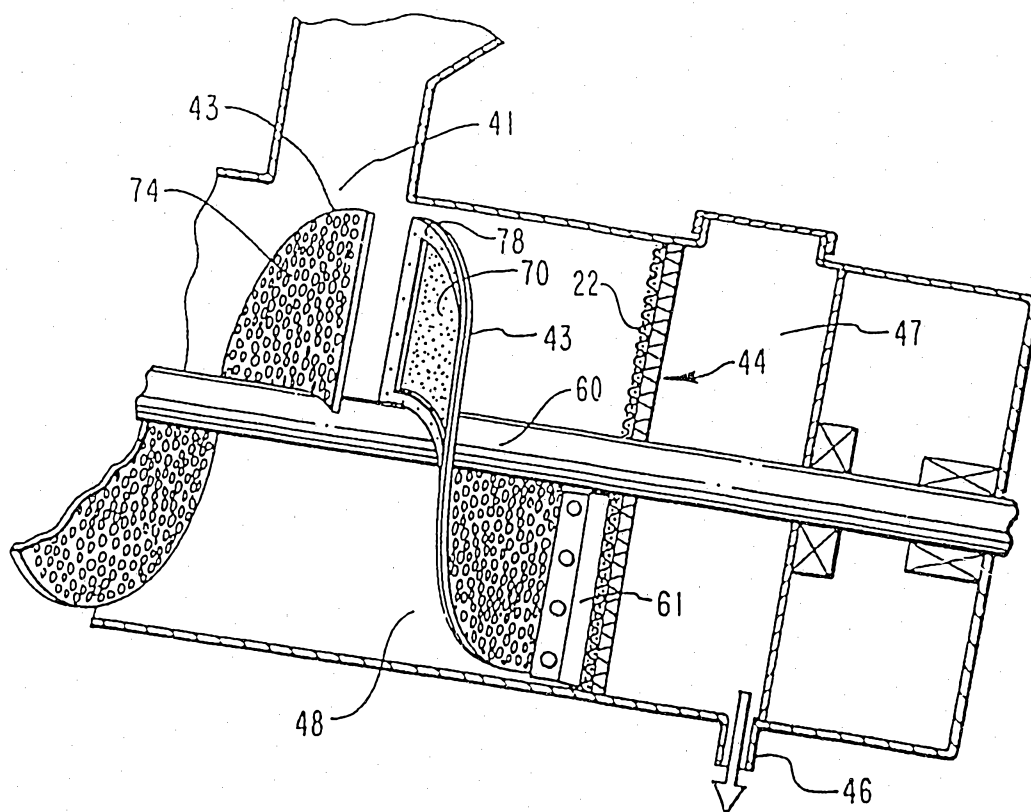
FIG. 4 EXTRACTION OUTLET
