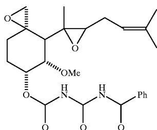
O-(N'-Benzoylallophanoyl)fumagillol
