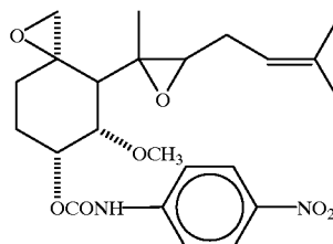
O-(p-Nitrophenylcarbamoyl)fumagillol
