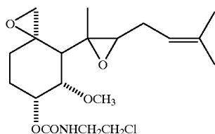
O-(2-Chloroethylcarbamoyl)fumagillol
