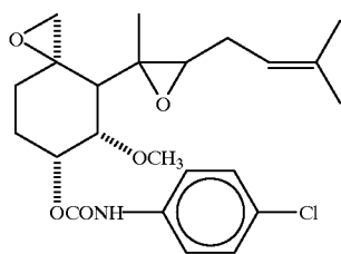
O-(p-Chlorophenylcarbamoyl)fumagillol
