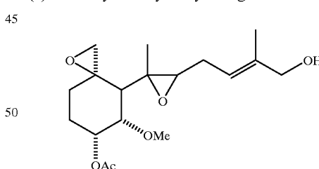
O-Chloroacetylcarbamoyl-6'b-dimethylaminofumagillol
