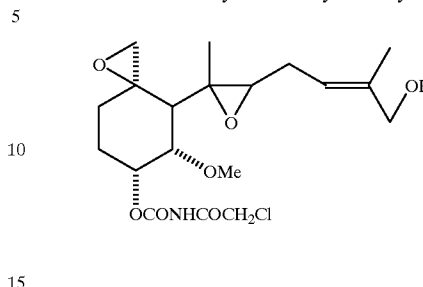
O-Chloroacetylcarbamoyl-6'b-hydroxyfumagillol
