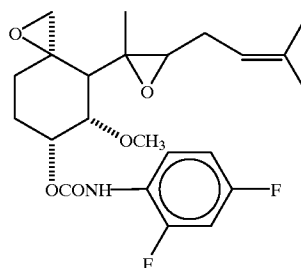
O-(2,4-Difluorophenylcarbamoyl)fumagillol
