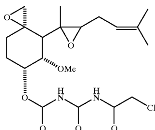
O-(N'-Chloroacetylallophanoyl)fumagillol
