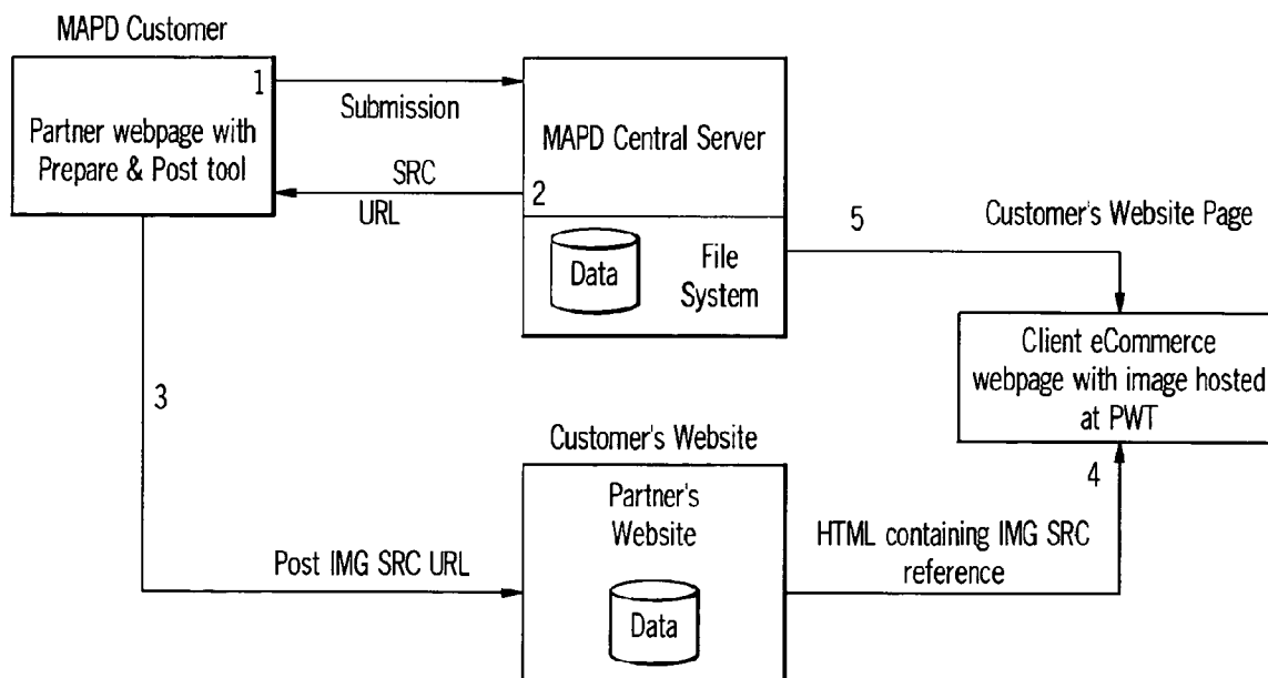
Host Service Transaction Flow
