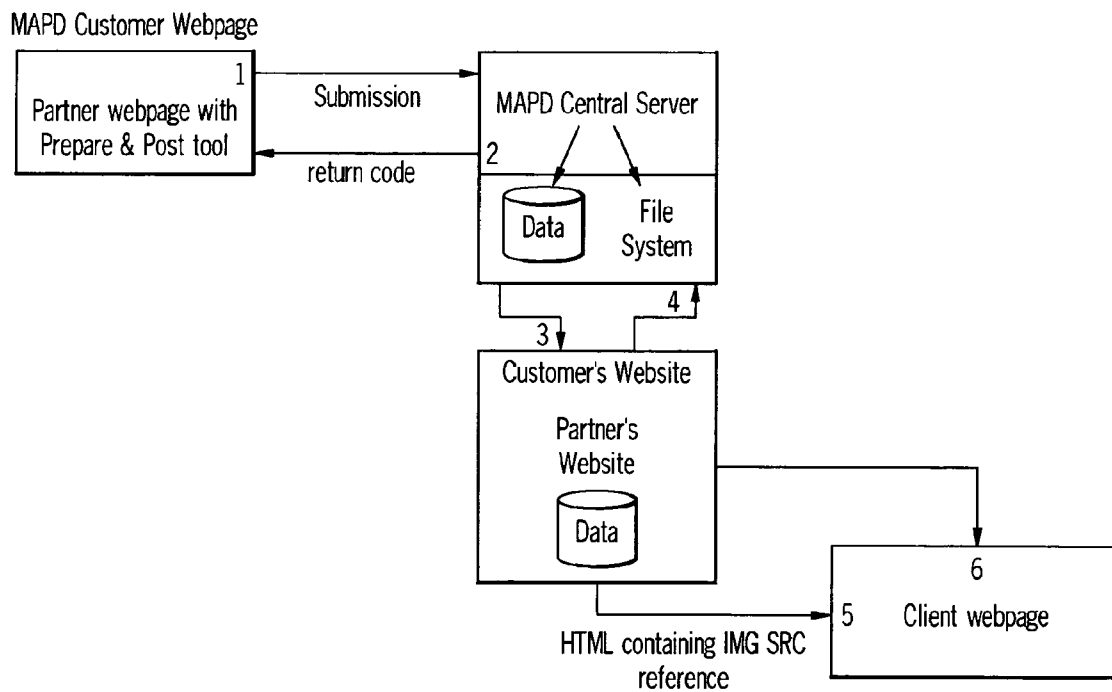
MIRROR Service Transaction Flow
