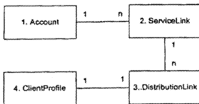
MIRROR Service Entities
