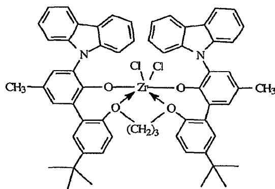
A10: bis((2-oxoyl-3-(dibenzo-1H-pyrrole-1-yl)-5-(methyl)phenyl)-(5-(2-methyl)propane-2-yl)-2-phenoxy)-1,3-propanediyl zirconium (IV) dichloride
