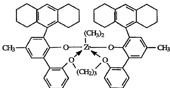
A1: bis((2-oxoyl-3-(1,2,3,4,6,7,8,9-octahydroanthracen-5-yl)-5-(methylphenyl)-2-phenoxy)-1,3-propanediyl zirconium (IV) dimethyl
