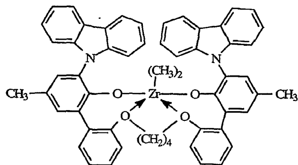
A8: bis((2-oxoyl-3-(dibenzo-1H-pyrrole-1-yl)-5-(methyl)phenyl)-2-phenoxy)-1,4-butanediylzirconium (IV) dimethyl
