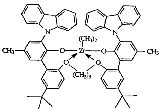
A9: bis((2-oxoyl-3-(dibenzo-1H-pyrrole-1-yl)-5-(methyl)phenyl)-(5-(2-methyl)propane-2-yl)-2-phenoxy)-1,3-propanediyl zirconium (IV) dimethyl
