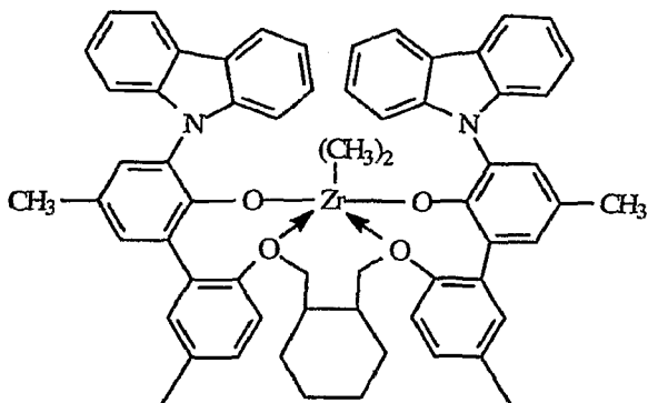
A7: bis((2-oxoyl-3-(dibenzo-1H-pyrrole-1-yl)-5-(methyl)phenyl)-(4-methyl-2-phenoxy)methyl)-trans 1,2-cyclohexanezirconium (IV) dimethyl
