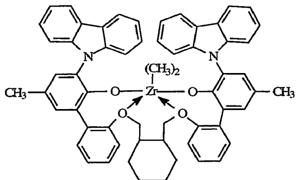
A2: bis((2-oxoyl-3-(dibenzo-1H-pyrrole-1-yl)-5-(methylphenyl)-2-phenoxy)-trans-1,2-cyclohexanediy zirconium (IV) dimethyl
