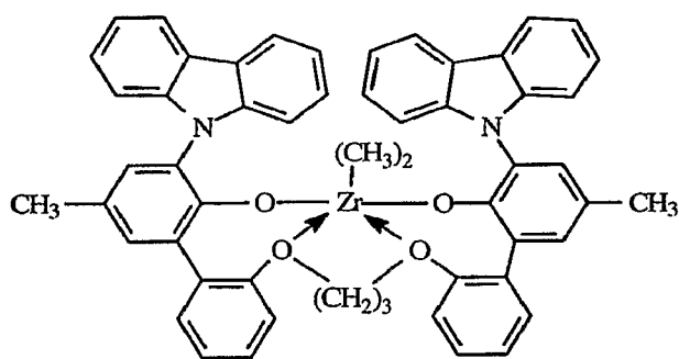
A4: bis((2-oxoyl-3-(dibenzo-1H-pyrrole-1-yl)-5-(methylphenyl)-2-phenoxy)-1,3-propanediyl zirconium (IV) dimethyl
