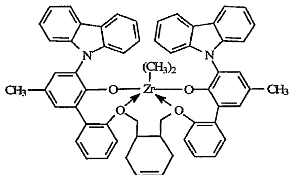
A6: bis((2-oxoyl-3-(dibenzo-1H-pyrrole-1-yl)-5-(methylphenyl)-2-phenoxy)-cis-4,5-cyclohexenediy zirconium (IV) dimethyl
