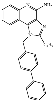
6b: 1-(Biphenyl-4-ylmethyl)-2-butyl-1H-imidazo[4,5-c]quinolin-4-amine
