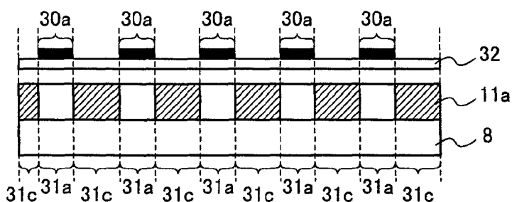
FIG. 15B (PRIOR ART) EXPOSURE
