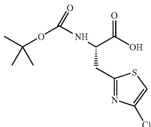
(S)-methyl 2-(tert-butoxycarbonyl)-3-(4-chlorothiazol-2-yl)propanoate
