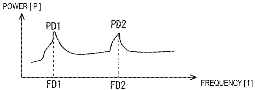
FREQUENCY SPECTRUM OF DOWN-BEAT FREQUENCY COMPONENTS
