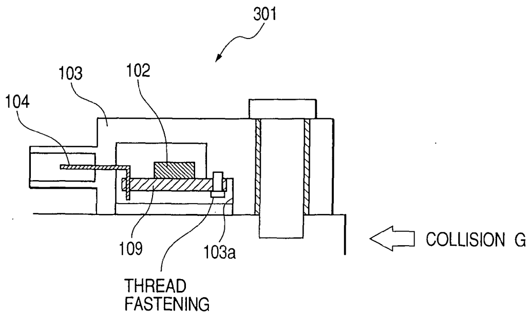
FIG. 18 COMPARATIVE ARRANGEMENT
