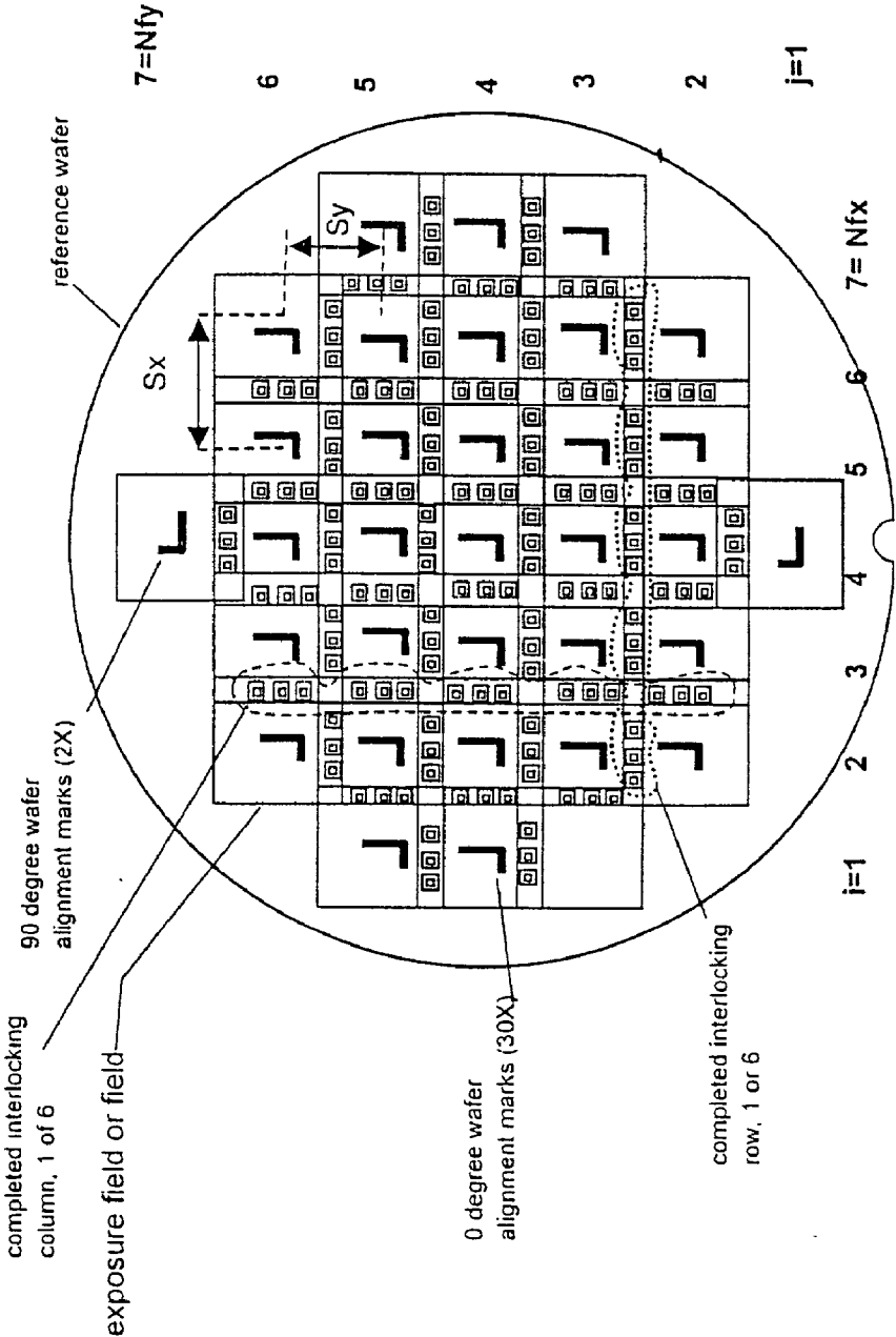
Figure 36 Tiled or interlocking schematic for reference wafer containing only wafer alignment marks and interlocking rows and columns.
