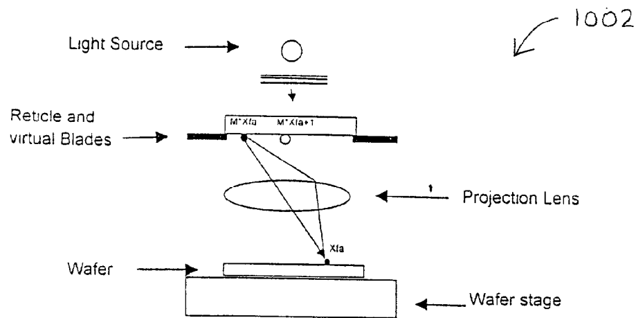
Figure 10 Photolithographic stepper or scanner system
