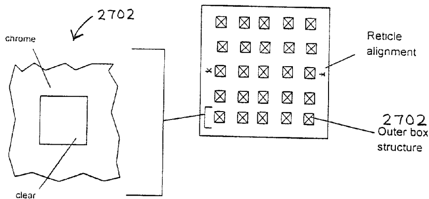
Figure 28 Outer box reticle detail
