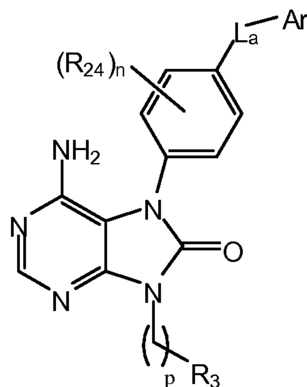
Formula (II);
