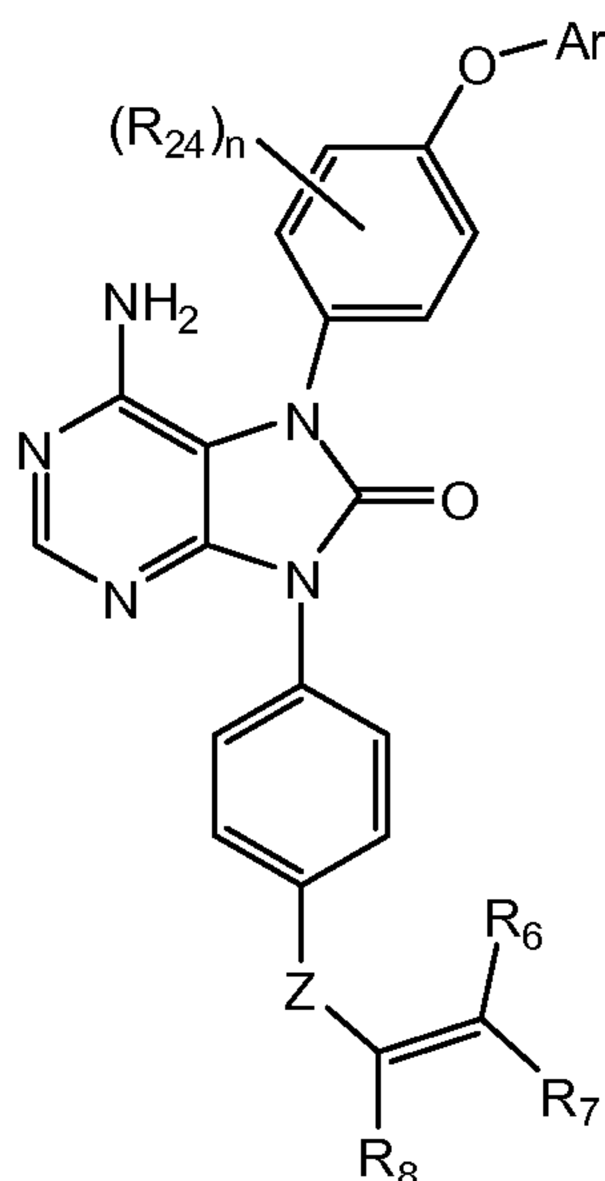
Formula (Ib);
