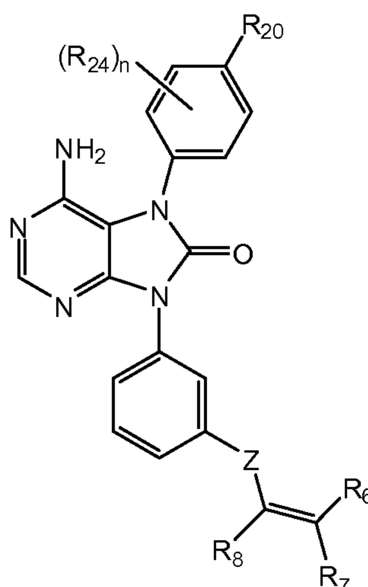
Formula (IIIa);
