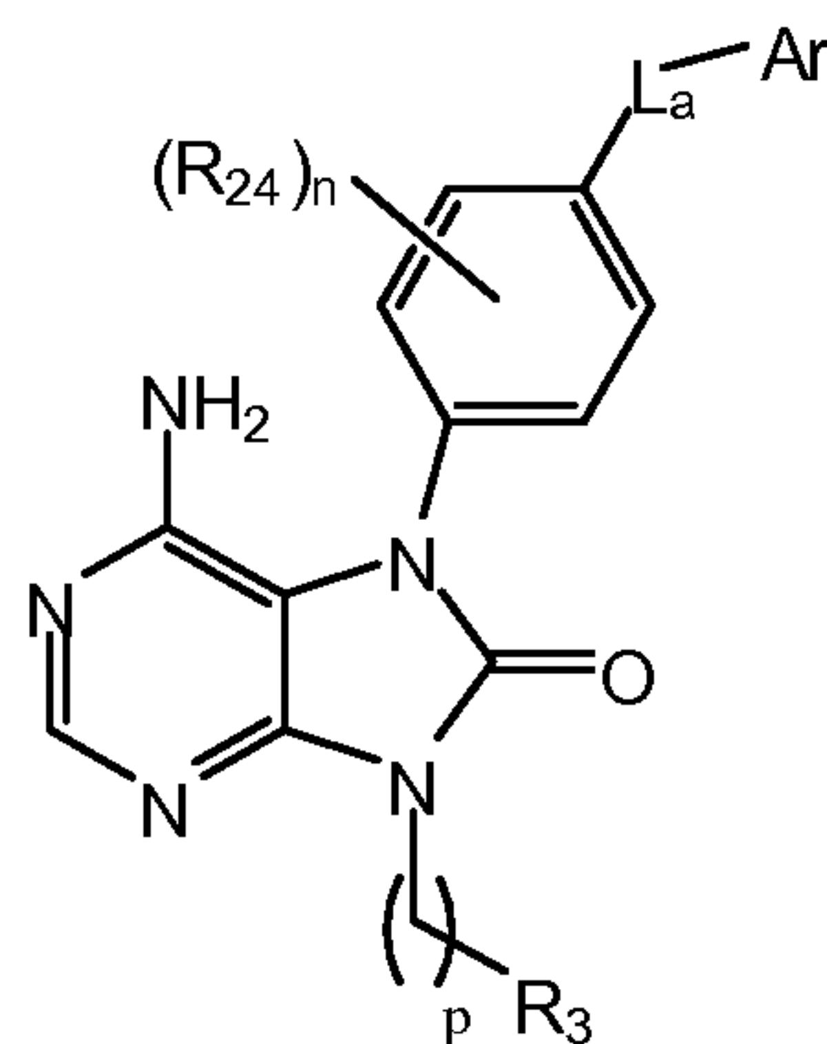
Formula (I);
