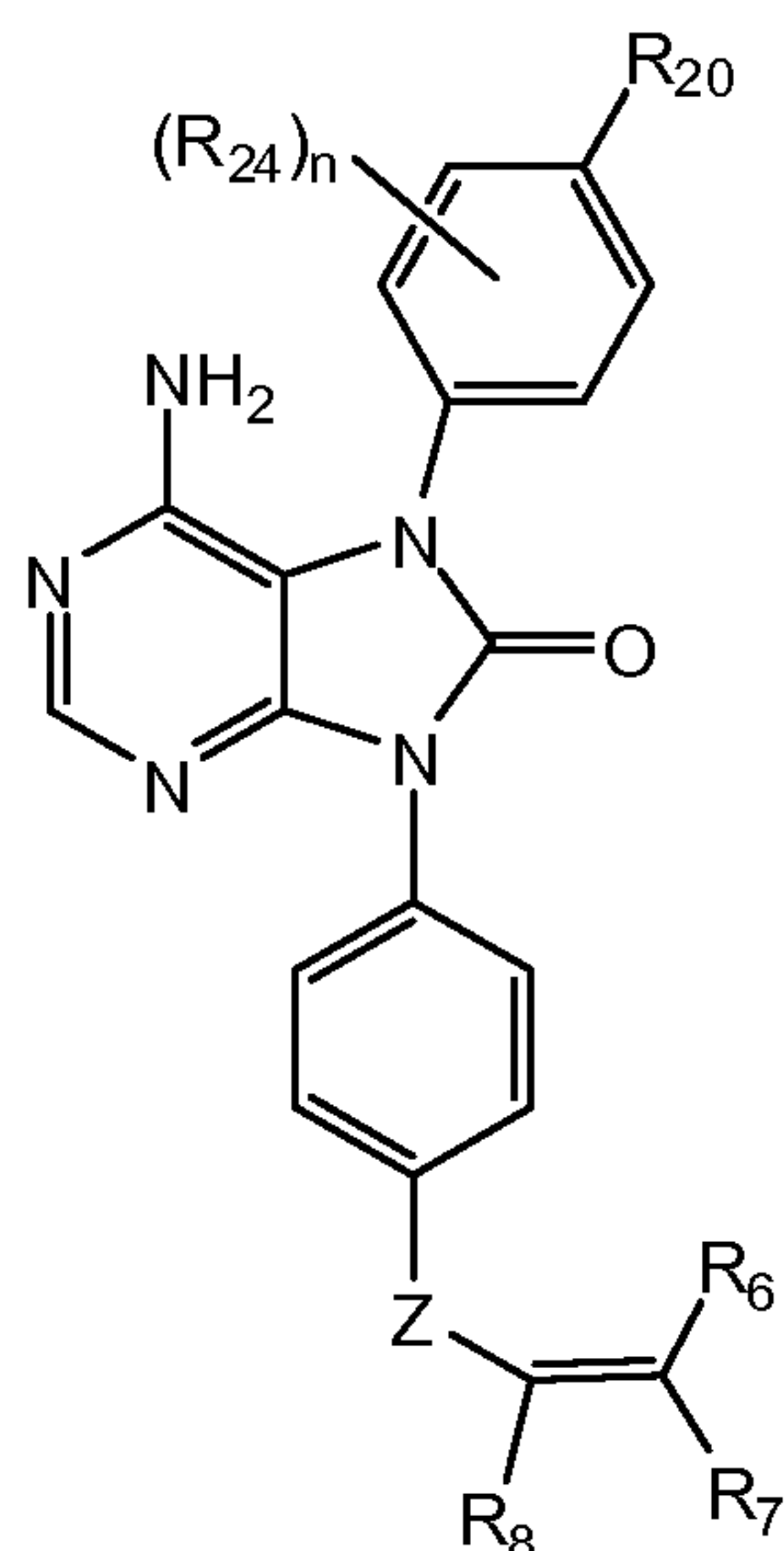
Formula (IIIb);
