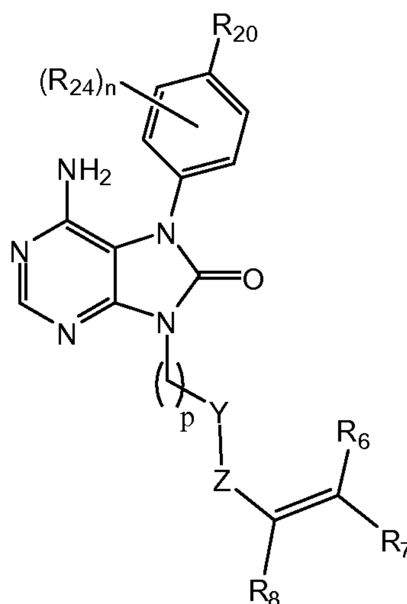
Formula (IIIc);
