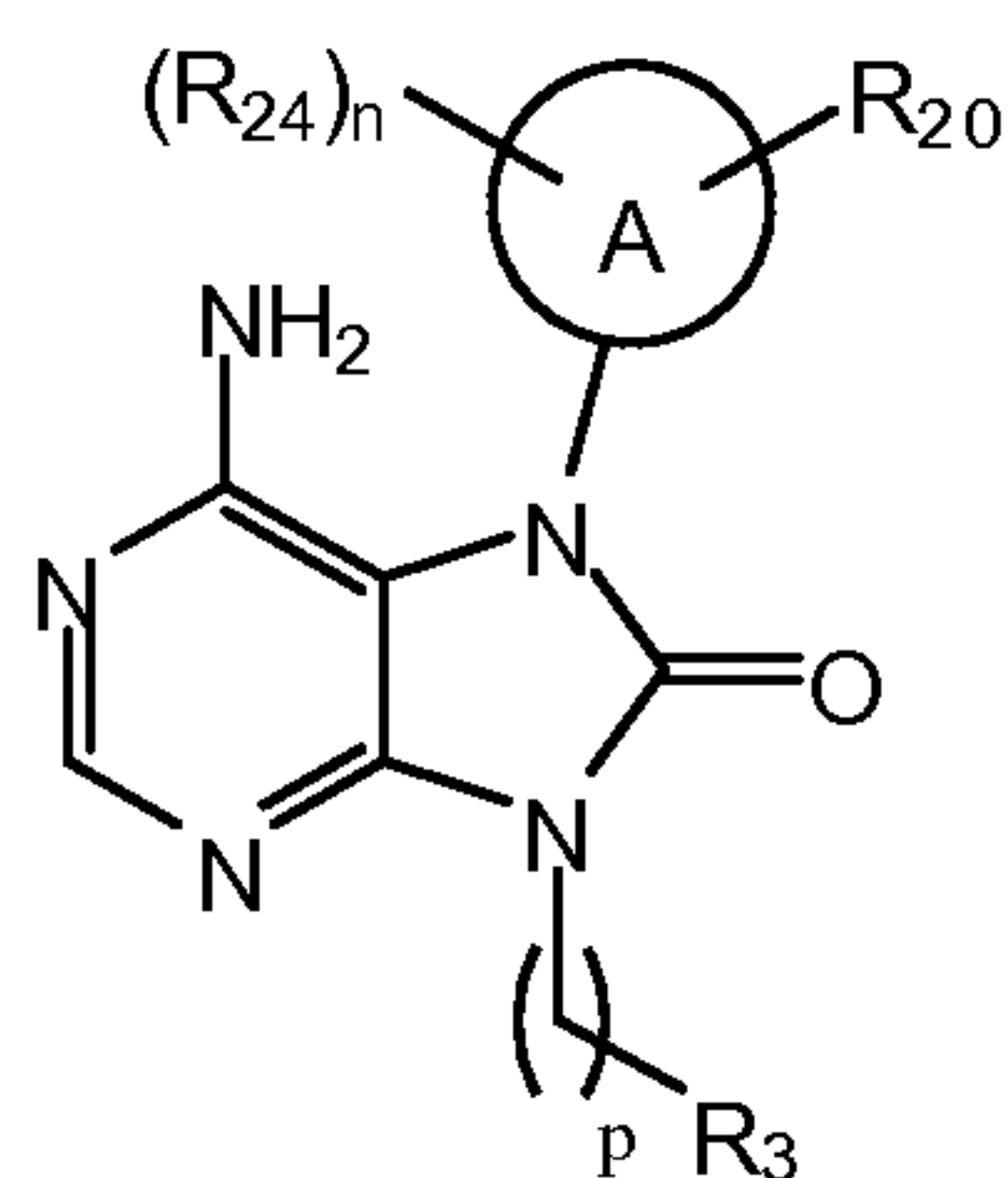
Formula (III);
