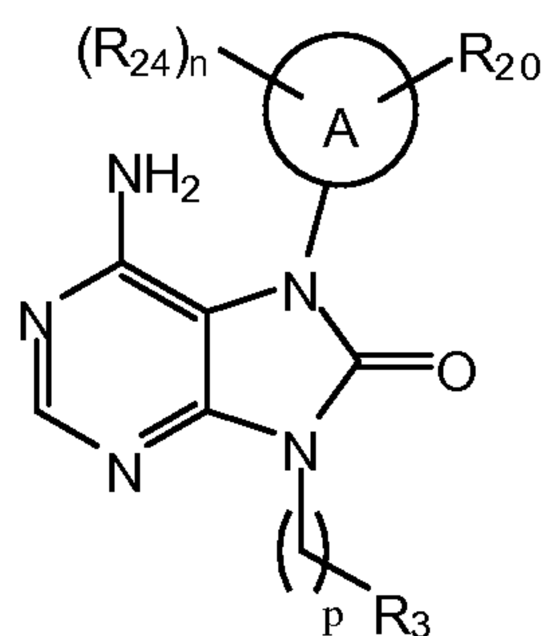
Formula (III);
