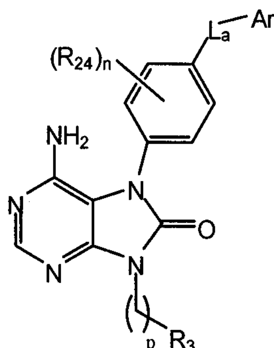
Formula (I);
