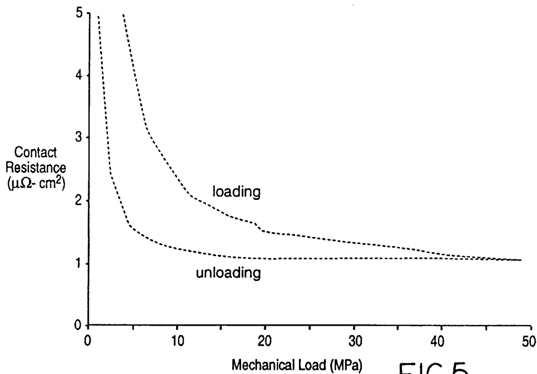
Mechanical Interconnection of ECB to Pd Surface
