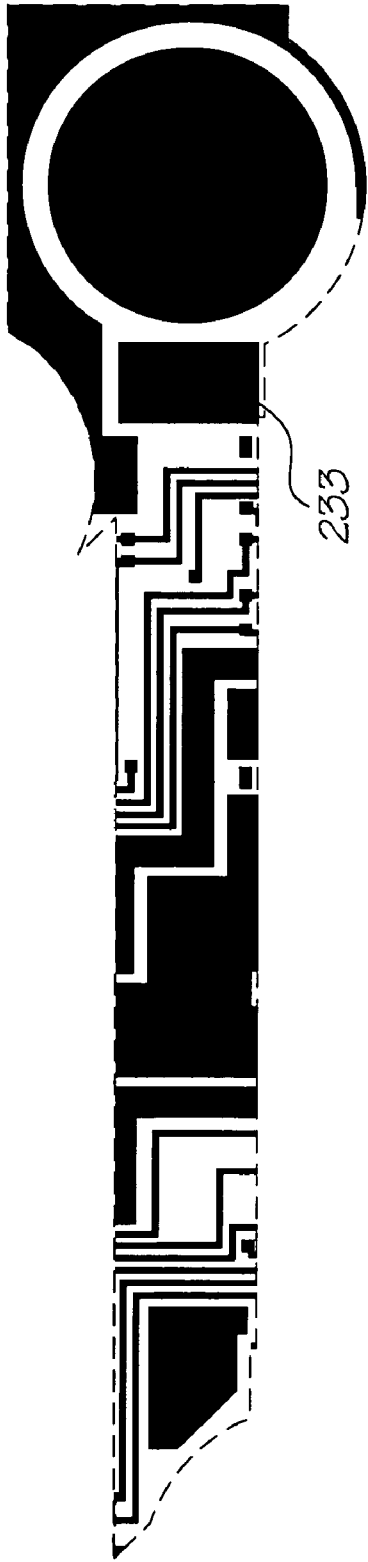
Metal 2 mask
