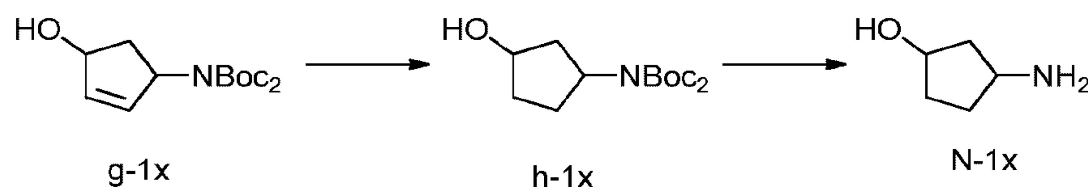
Scheme VIII
