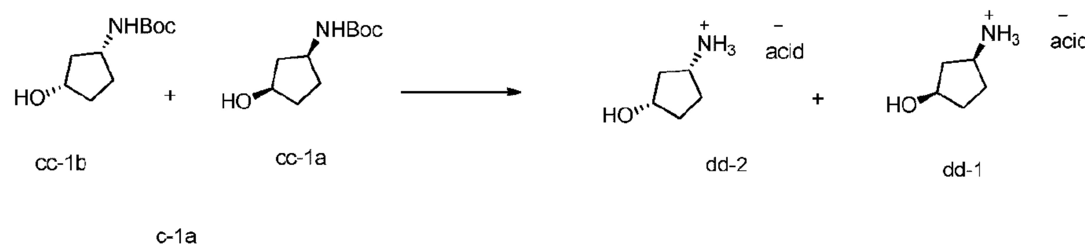
Scheme XI
