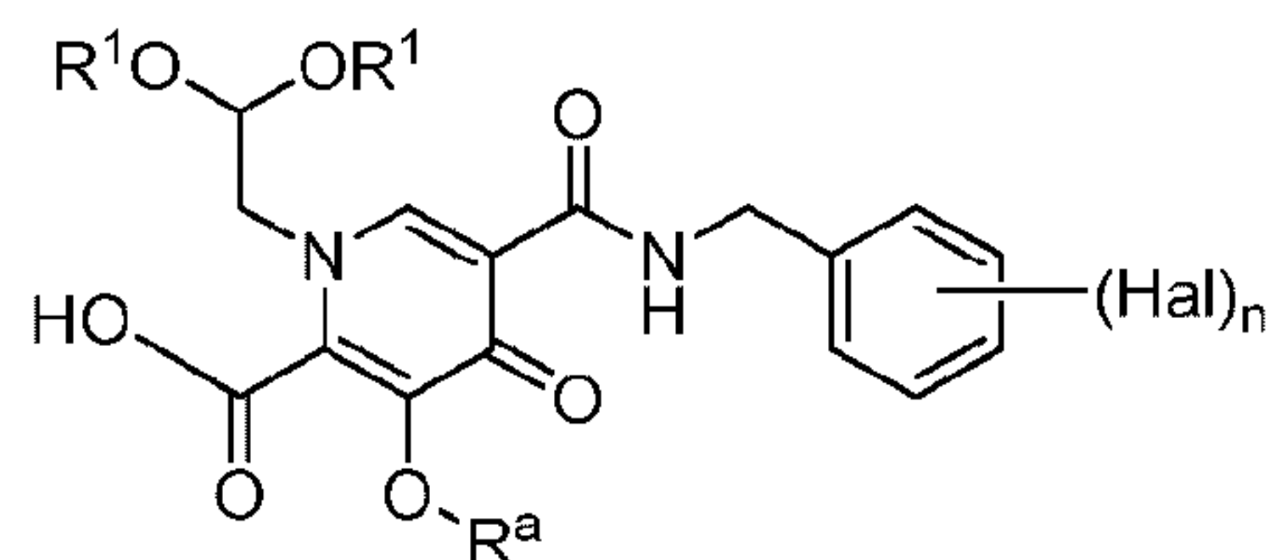
II
