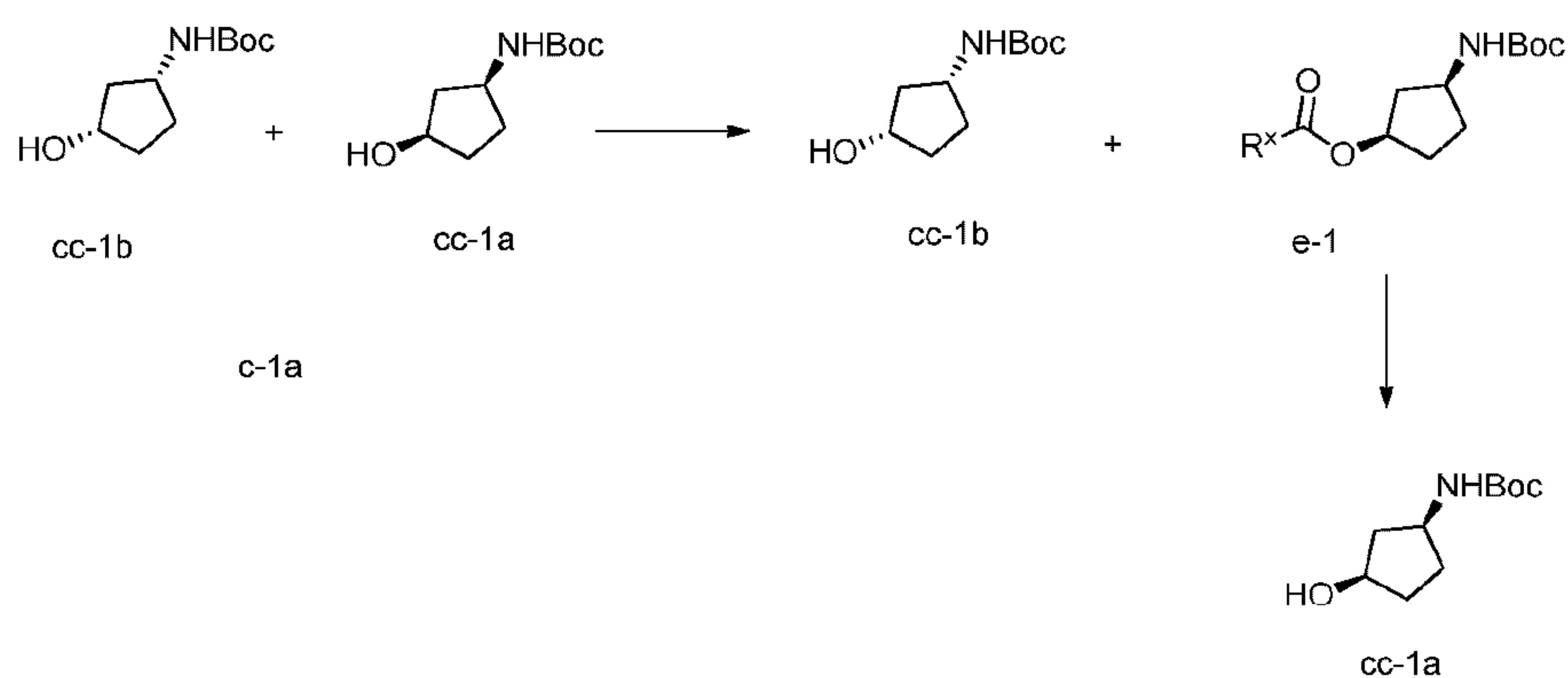
Scheme IX
