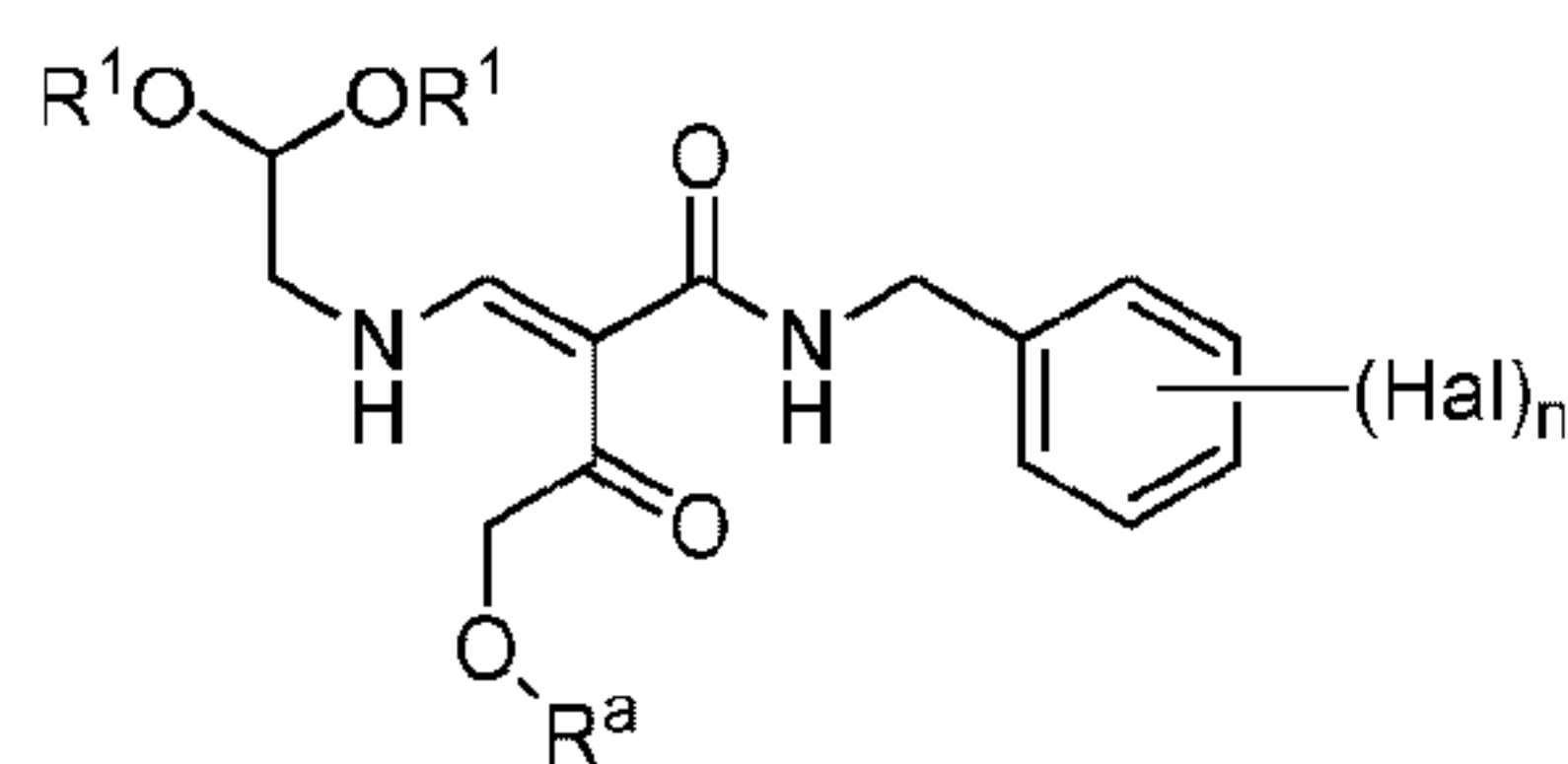
(E-1) (E)-configuration
