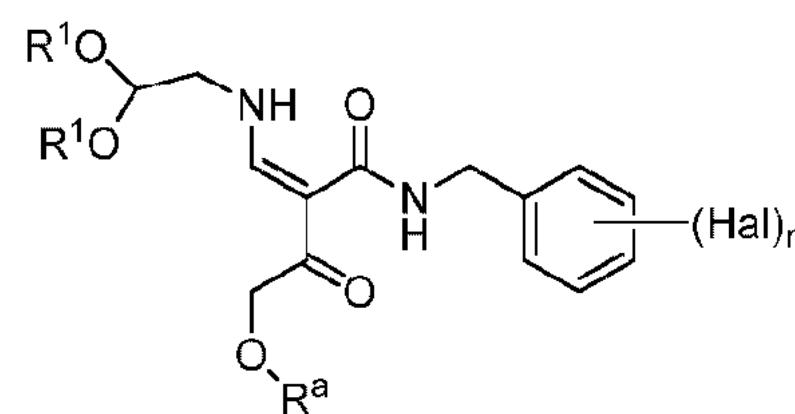
(E-1) (Z)-configuration
