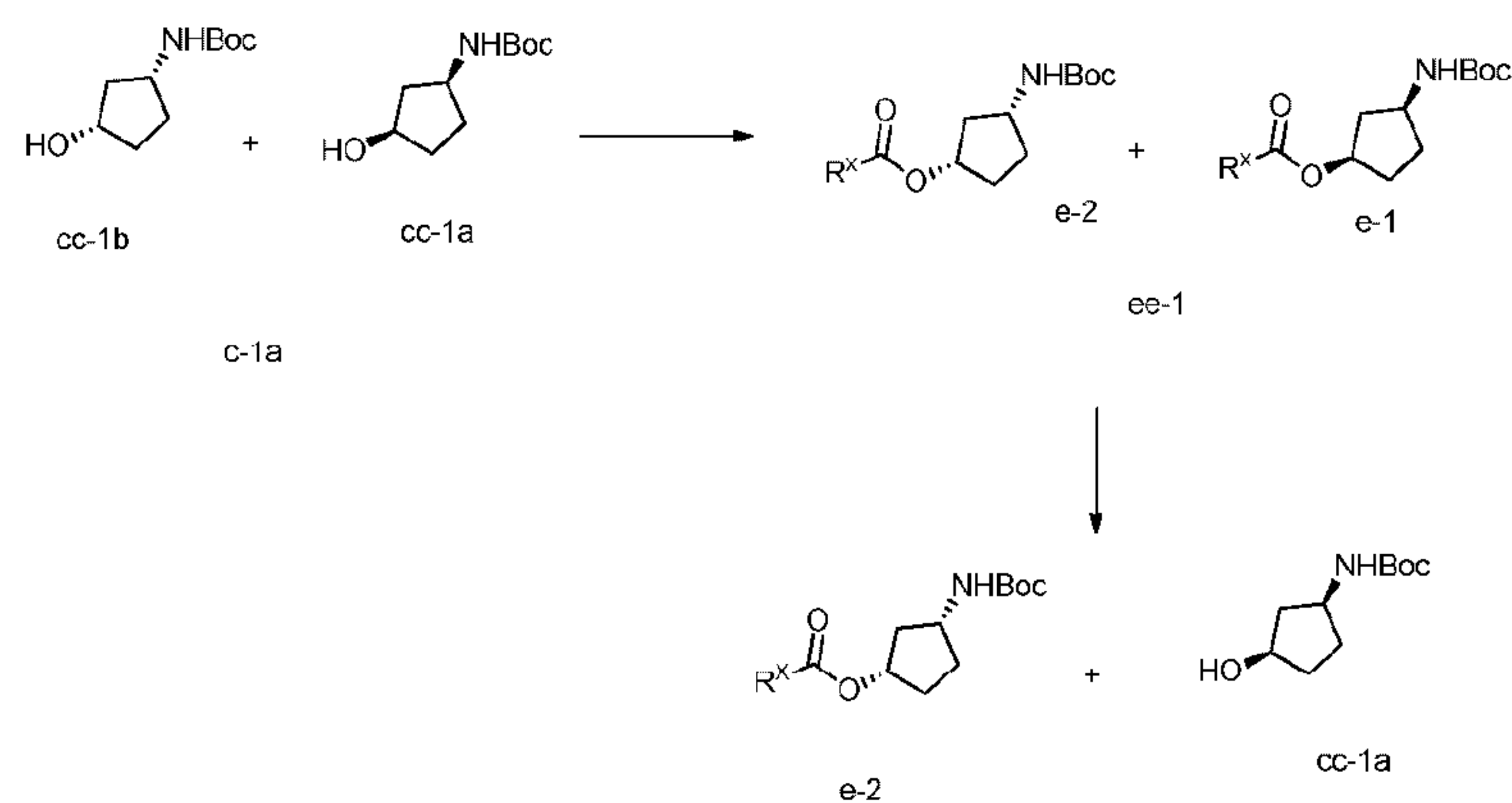
Scheme X
