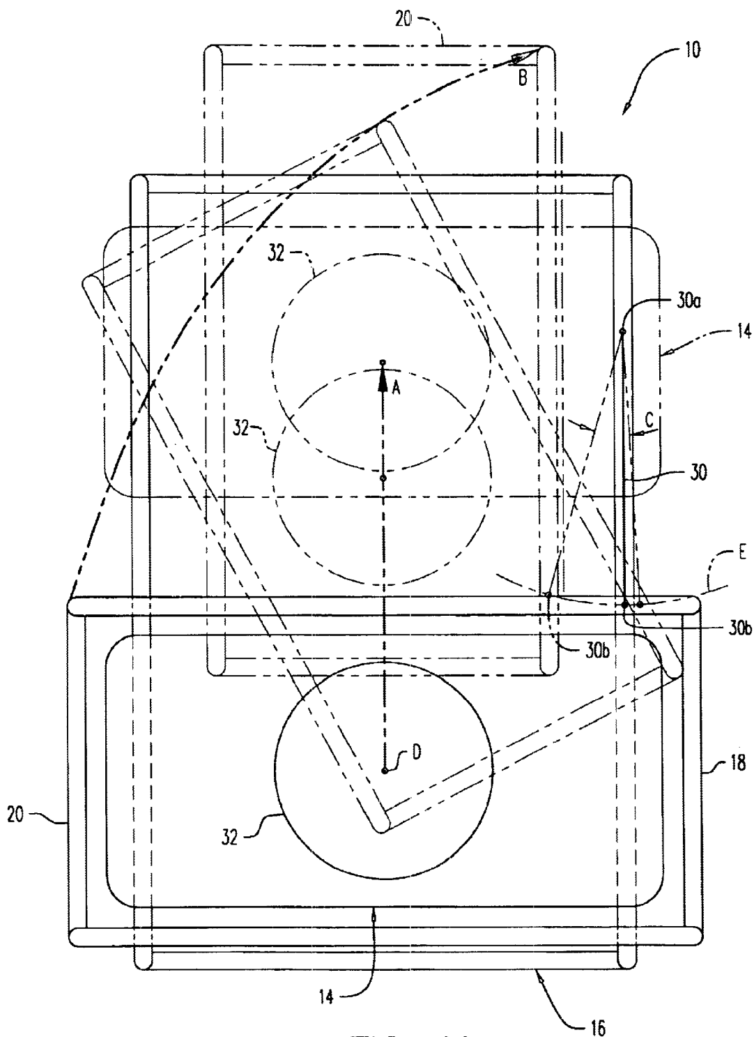
FIG. 11 (PRIOR ART)
