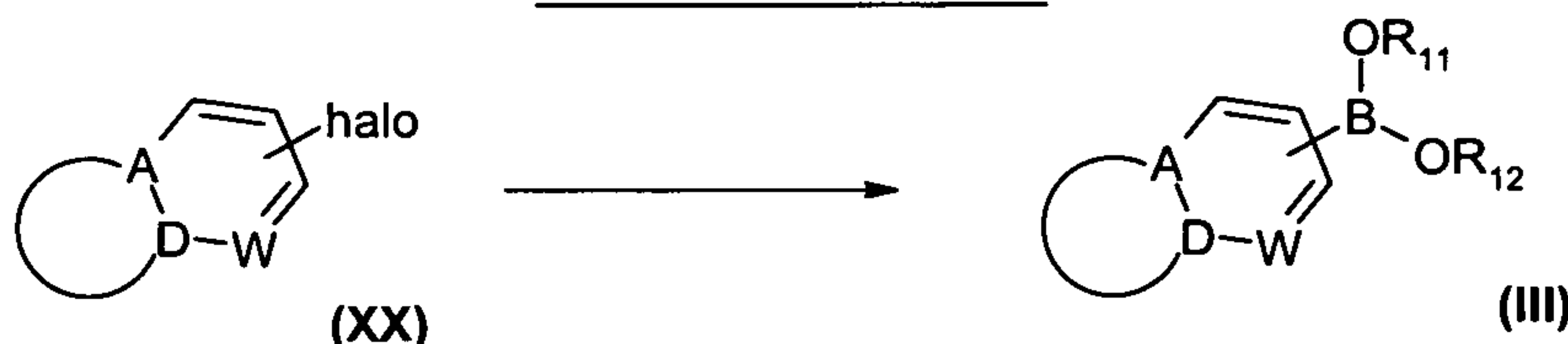
Reaction Scheme 20
