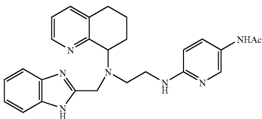
Compound 14: Preparation of N-(6-2-[(1H-Benzimidazol-2-ylmethyl)-(5,6,7,8-tetrahydro-quinolin-8-yl)-amino]-ethylamino)-1-pyridin-3-yl)-acetamide
