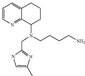
Compound 126: \text{N}^1 -(4-methyl-1H-imidazol-2-ylmethyl)- \text{N}^1 -(5,6,7,8-tetrahydro-quinolin-8-yl)-butane-1,4-diamine (Hydrobromide Salt)
