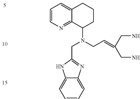
Compound 79: 3-Aminomethyl-N'-(1H-benzimidazol-2-ylmethyl)-N'-(5,6,7,8-tetrahydroquinolin-8-yl)-but-2-ene-1,4-diamine (Hydrobromide Salt)
