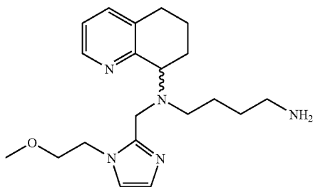
Compound 128: Preparation of \text{N}^1 -[1-(2-methoxy-ethyl)-1H-imidazol-2-ylmethyl]- \text{N}^1 -(5,6,7,8-tetrahydro-quinolin-8-yl)-butane-1,4-diamine (Hydrobromide Salt)
