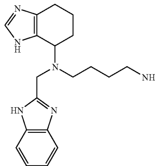
Compound 110: \text{N}^1 -(1H-Benzoimidazol-2-ylmethyl)- \text{N}^1 -(4,5,6,7-tetrahydro-3H-benzoimidazol-4-yl)-butane-1,4-diamine (Hydrobromide Salt)
