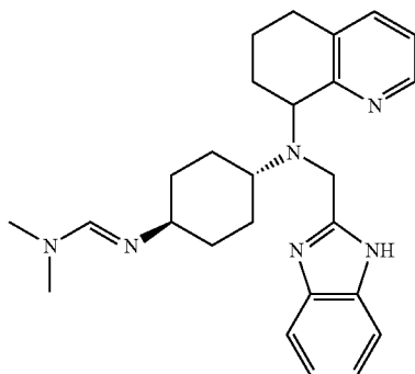
Compound 63: Preparation of 1-N'-[trans-4-(1H-Benzimidazol-2-ylmethyl)-(5,6,7,8-tetrahydroquinolin-8-yl)-amino]-cyclohexanyl-N,N-dimethylformamide (Hydrobromide Salt)
