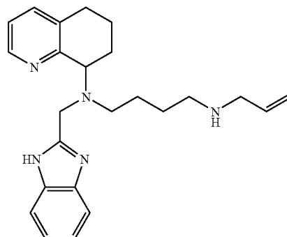
Compound 33: (1H-Benzimidazol-2-ylmethyl)-(5,6,7,8-tetrahydroquinolin-8-yl)-(N-allyl-4-amino-but-1-yl)-amine
