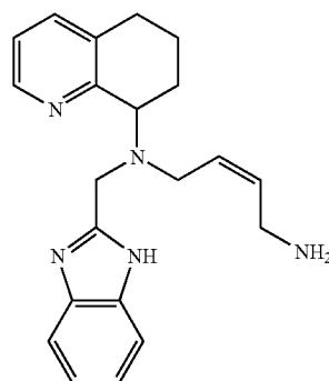
Compound 74: Preparation of (Z)-N 1 -(1H-Benzimidazol-2-ylmethyl)-N 4 -(5,6,7,8-tetrahydro-quinolin-8-yl)-but-2-ene-1,4-diamine
