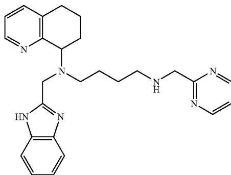
Compound 29: Preparation of N-(1H-benzimidazol-2-ylmethyl)-N'-pyrimidin-2-ylmethyl-N'-(5,6,7,8-tetrahydroquinolin-8-yl)-butane-1,4-diamine (Hydrobromide Salt).
