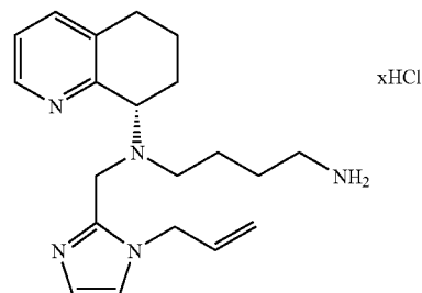
Compound 135: Preparation of N 1 -(1-Allyl-1H-imidazol-2-ylmethyl)-N 1 -(S)-5,6,7,8-tetrahydro-quinolin-8-yl-butane-1,4-diamine (Hydrochloride Salt)
