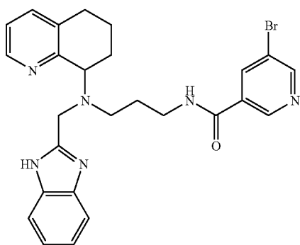
Compound 143: N-{3-[(1H-benzoimidazol-2-ylmethyl)-(5,6,7,8-tetrahydro-quinolin-8-yl)-amino]-propyl}-5-bromo-nicotinamide
