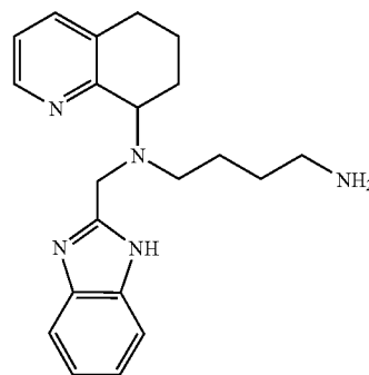
Compound 17: Preparation of N¹-(1H-Benzimidazol-2-ylmethyl)-N¹-(5,6,7,8-tetrahydroquinolin-8-yl)-butane-1,4-diamine (Hydrobromide Salt)
