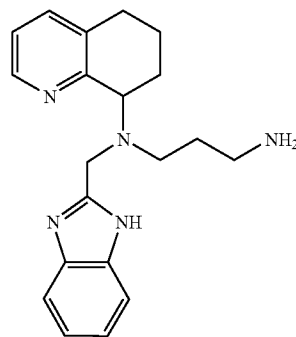
Compound 15: Preparation of N¹-(1H-Benzimidazol-2-ylmethyl)-N¹-(5,6,7,8-tetrahydroquinolin-8-yl)-propane-1,3-diamine (Hydrobromide Salt)
