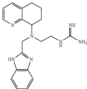
Compound 136: Preparation of N 1 -{2-[(1H-Benzimidazol-2-ylmethyl)-N 1 -(5,6,7,8-tetrahydroquinolin-8-yl)-amino]-ethyl}-guanidine (Hydrobromide Salt)
