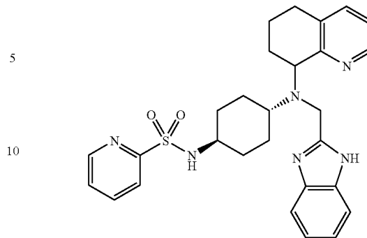
Compound 64: Preparation of N'-(1H-benzimidazol-2-ylmethyl)-N'-(5,6,7,8-tetrahydroquinolin-8-yl)-cyclohexane-trans-1,4-diamine-N-(2-pyridinyl)-sulfonamide
