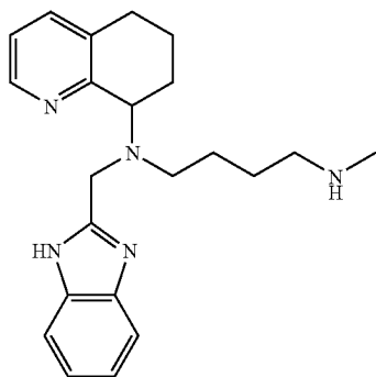
Compound 34: (1H-Benzimidazol-2-ylmethyl)-(5,6,7,8-tetrahydroquinolin-8-yl)-(N-methyl-4-amino-but-1-yl)-amine
