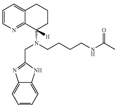
Compound 162: Preparation of N'-[4-[(1H-Benzimidazol-2-ylmethyl)-(S)-5,6,7,8-tetrahydroquinolin-8-yl-amino]-butyl]-acetamide (Free Base)
