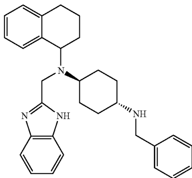
COMPOUND 56: Preparation of N¹-(1H-Benzimidazol-2-ylmethyl)-N¹-(5,6,7,8-tetrahydro-quinolin-8-yl)-N²-benzyl-cyclohexane-trans-1,4-diamine (Hydrobromide Salt)
