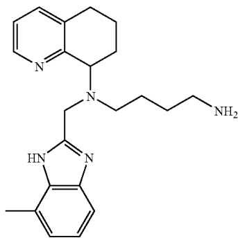
Compound 115: N 1 -(4-methyl-1H-benzimidazol-2-ylmethyl)-N 1 -(5,6,7,8-tetrahydro-quinolin-8-yl)-butane-1,4-diamine
