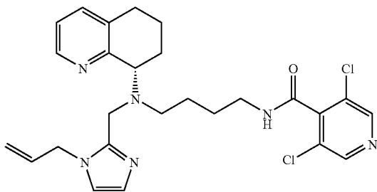
Compound 156: Preparation of N-{4-[(1-allyl-1H-imidazol-2-ylmethyl)-(S)-5,6,7,8-tetrahydro-quinolin-8-ylamino]-butyl}-3,5-dichloro-isonicotinamide
