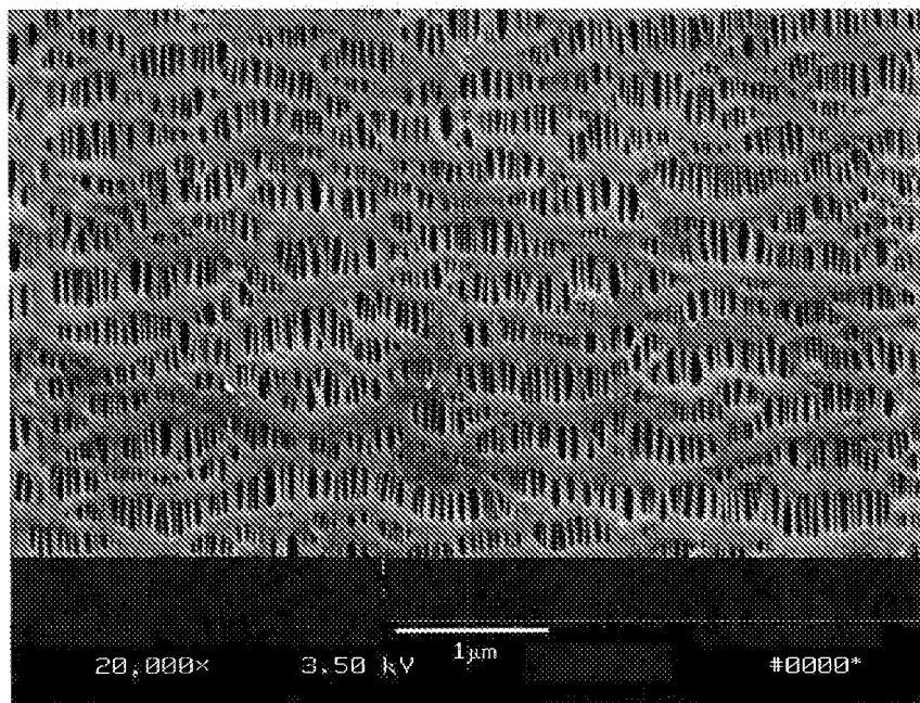
Figure 8. SEM of Surface of Ex. 3 Membrane.
