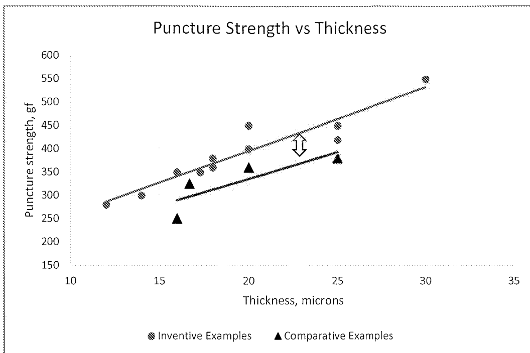
Figure 15. Puncture Strength vs. Thickness
