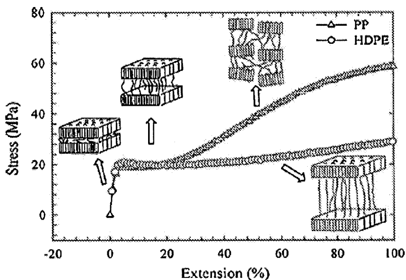
Figure 2. Stress Strain plot of PP and HDPE Membranes ((X.M. Zhang, et. al., "Oriented Structure and Anisotropy Properties of Polymer Blown Films HDPE, LLDPE and LDPE", POLYMER 45 (2004) 217–2291).
