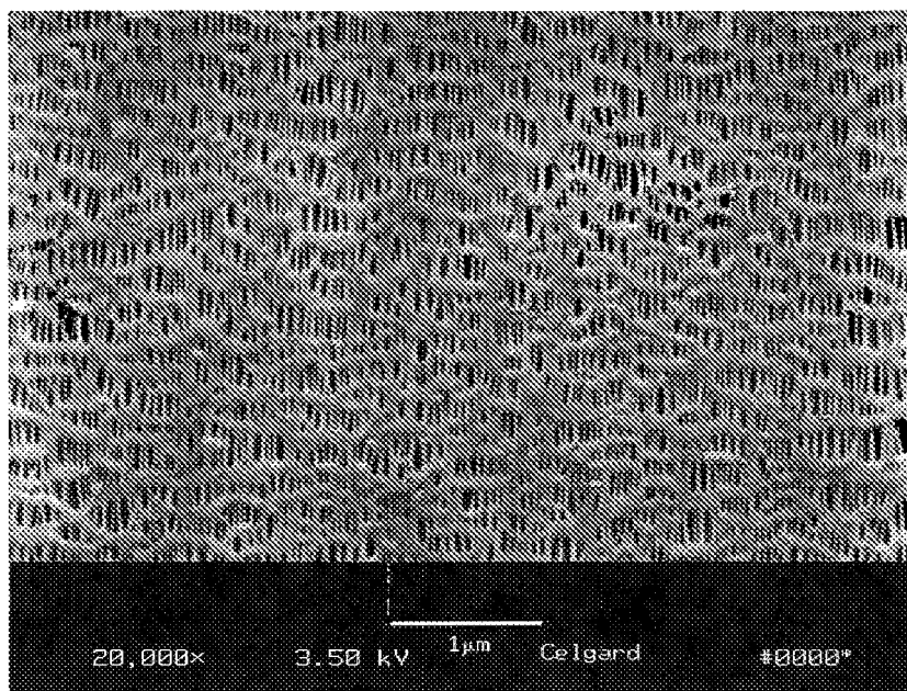
Figure 9. SEM of Surface of Ex. 4 Membrane.
