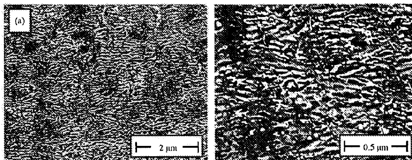
Figure 1. SEM Micrograph Surface of an Etched PP Membrane Showing Uniform and Ordered Stacked Lamellar Structure at Two Magnifications. (X.M. Zhang, et. al., "Oriented Structure and Anisotropy Properties of Polymer Blown Films HDPE, LLDPE and LDPE", POLYMER 45 (2004) 217-2291).
