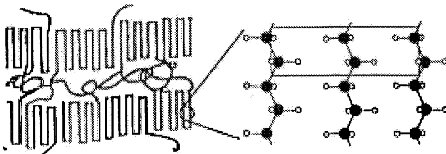
Figure 5. Schematic diagram of chain folding in polypropylene and the molecular level polymer structure in the folds. Ref: 'The Theory of Birefringence', Cambridge Polymer Group, 2004, CPGAN # 014, www.campoly.com .
