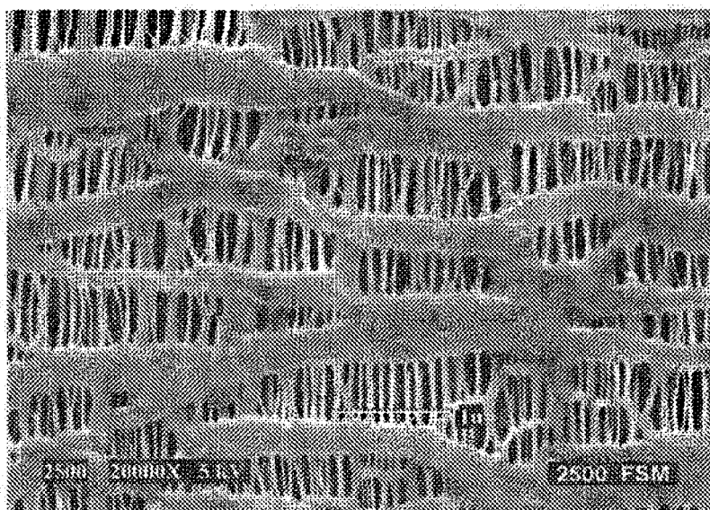
Figure 3. SEM of Surface of CE 6 Microporous Film at 20,000x Magnification.
