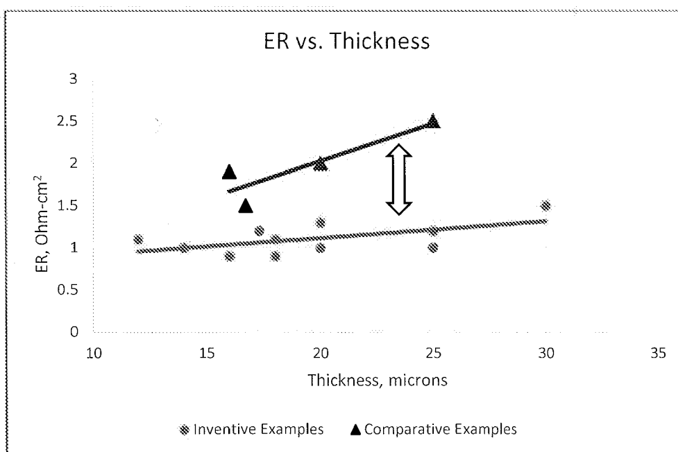
Figure 14. ER vs Thickness
