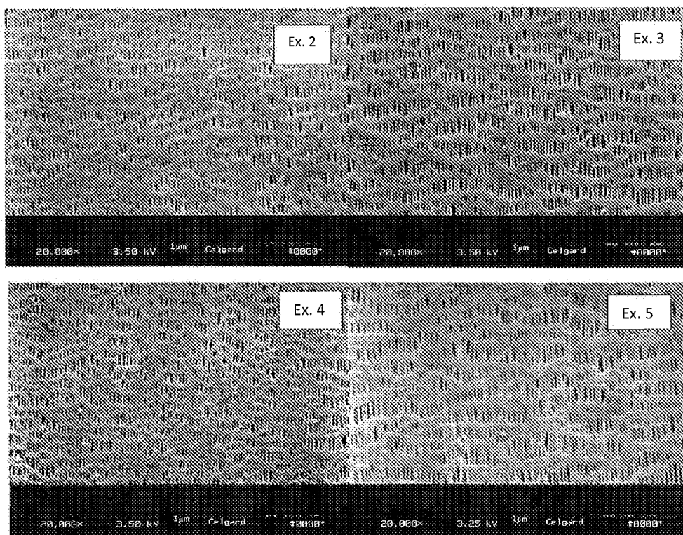
Figure 12. Side by Side Comparison of SEM Micrographs of Inventive Ex. 2, 3, 4 and 5 Membranes.
