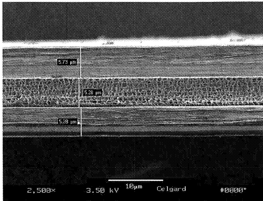
Figure 7. SEM of Cross Section View of Ex. 2 Membrane.
