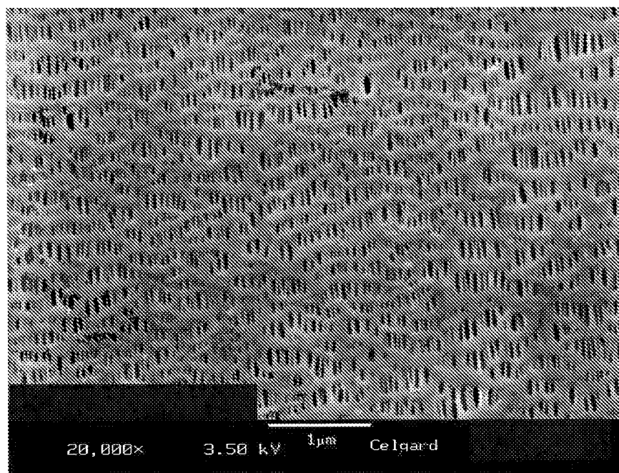
Figure 6. SEM of Surface of Ex. 2 Membrane.
