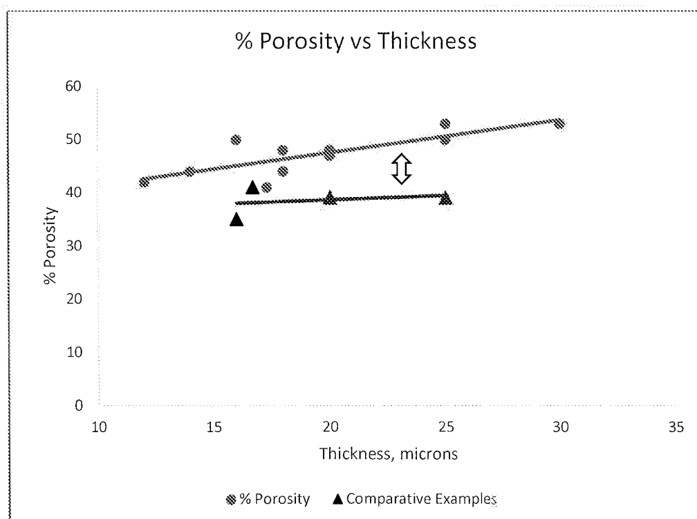
Figure 16. % Porosity vs. Thickness
