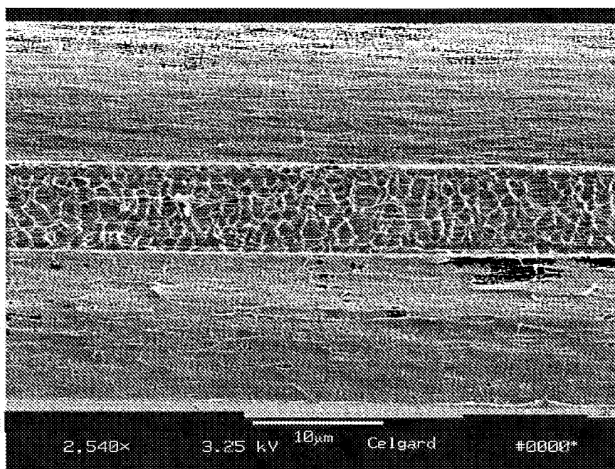
Figure 11. SEM of Cross Section View of Ex. 5 Membrane.
