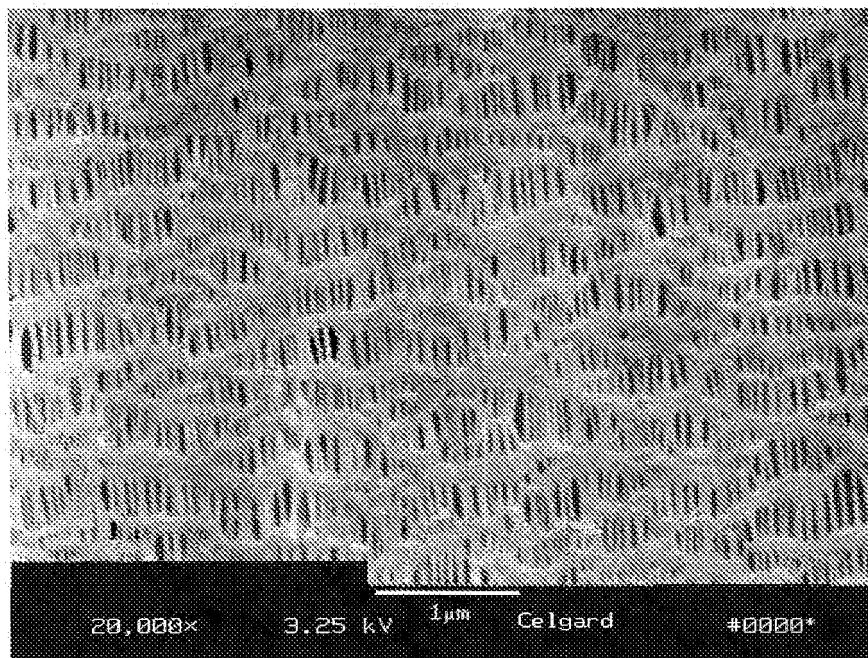
Figure 10. SEM of Surface of Ex. 5 Membrane.
