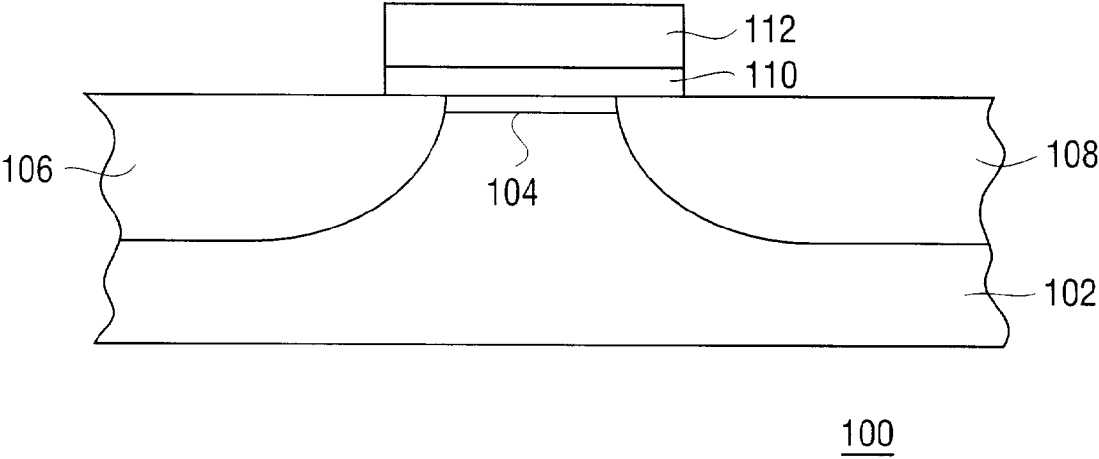
FIG. 1 (PRIOR ART)
