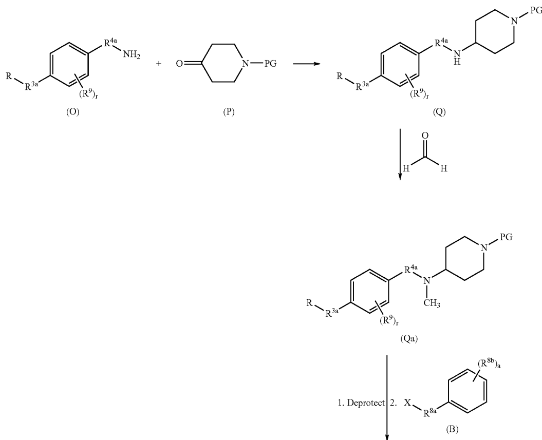
REACTION SCHEME 5
