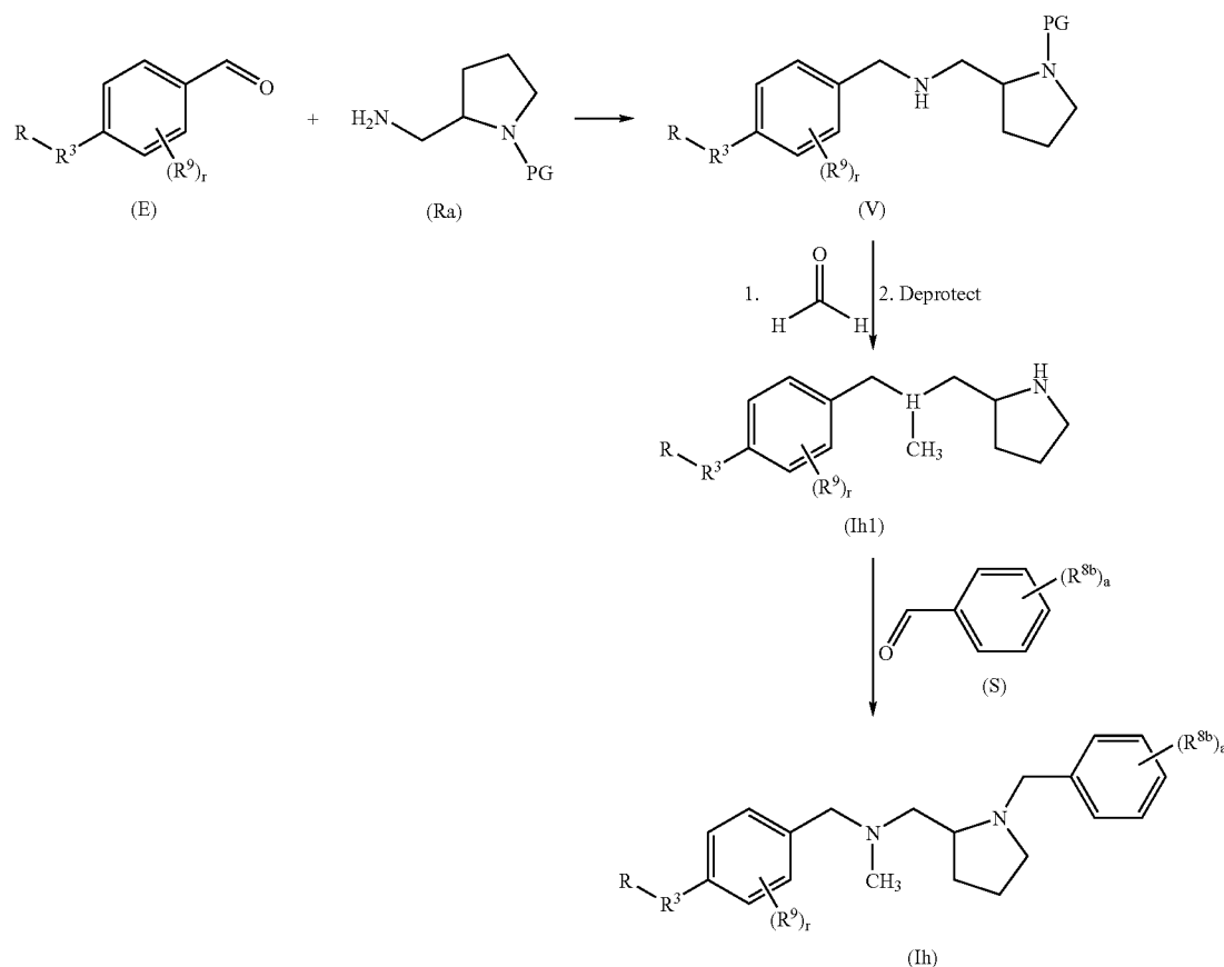
REACTION SCHEME 8
