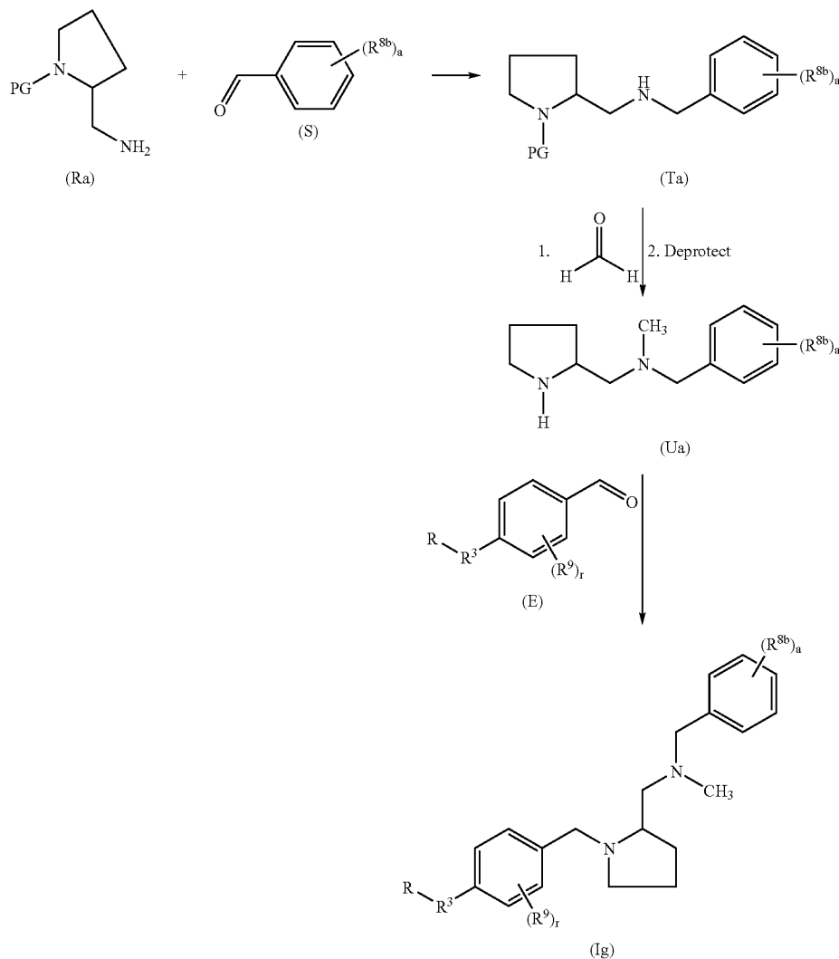
REACTION SCHEME 7
