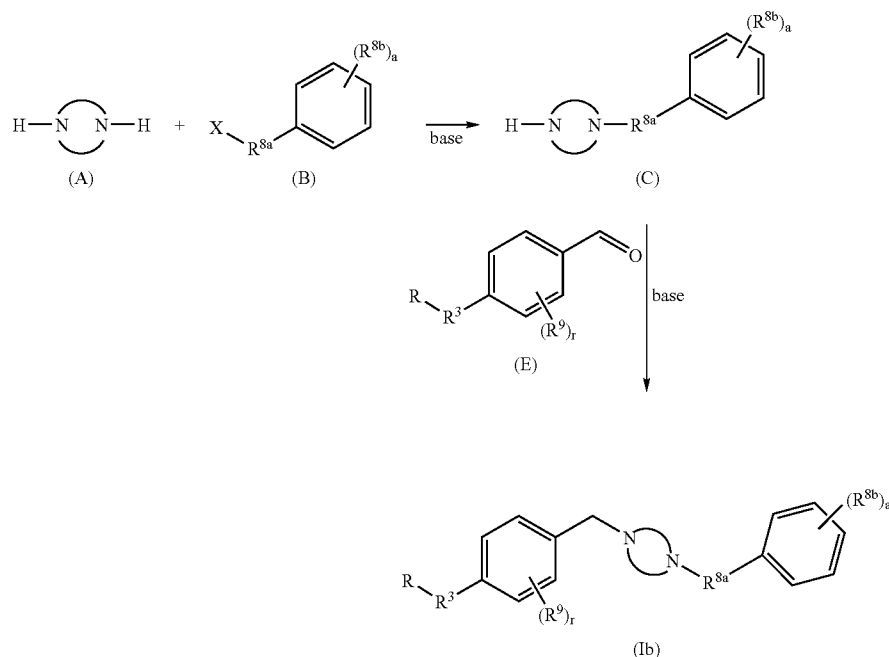
REACTION SCHEME 2
