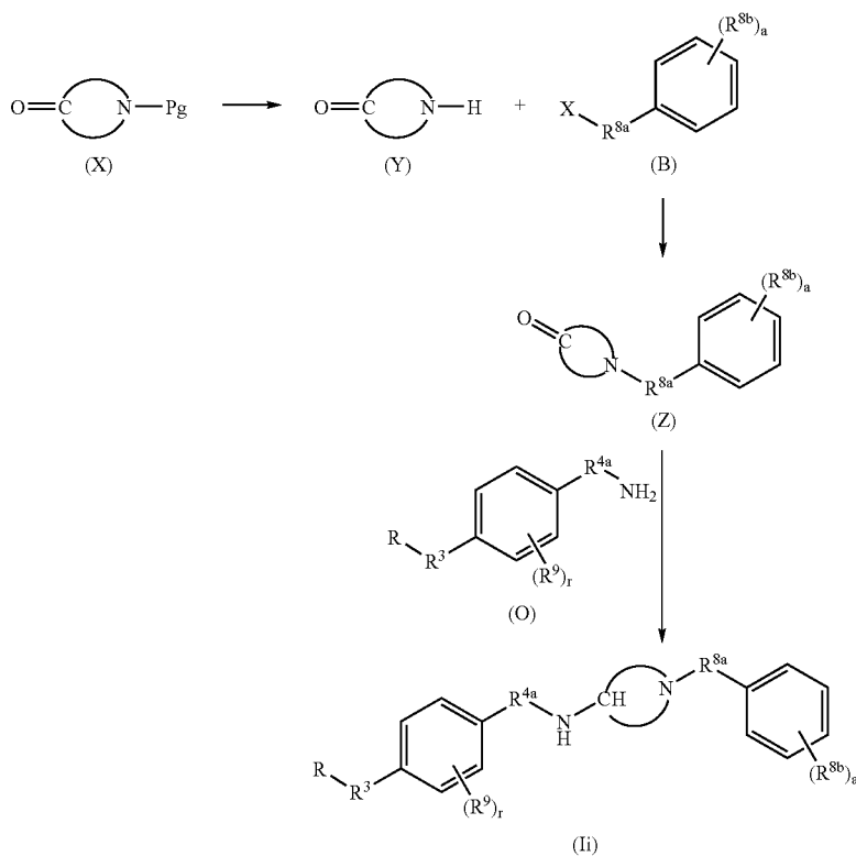
REACTION SCHEME 9
