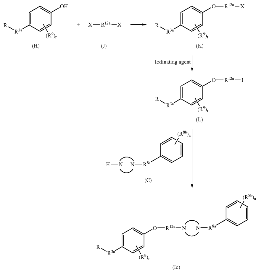
REACTION SCHEME 3
