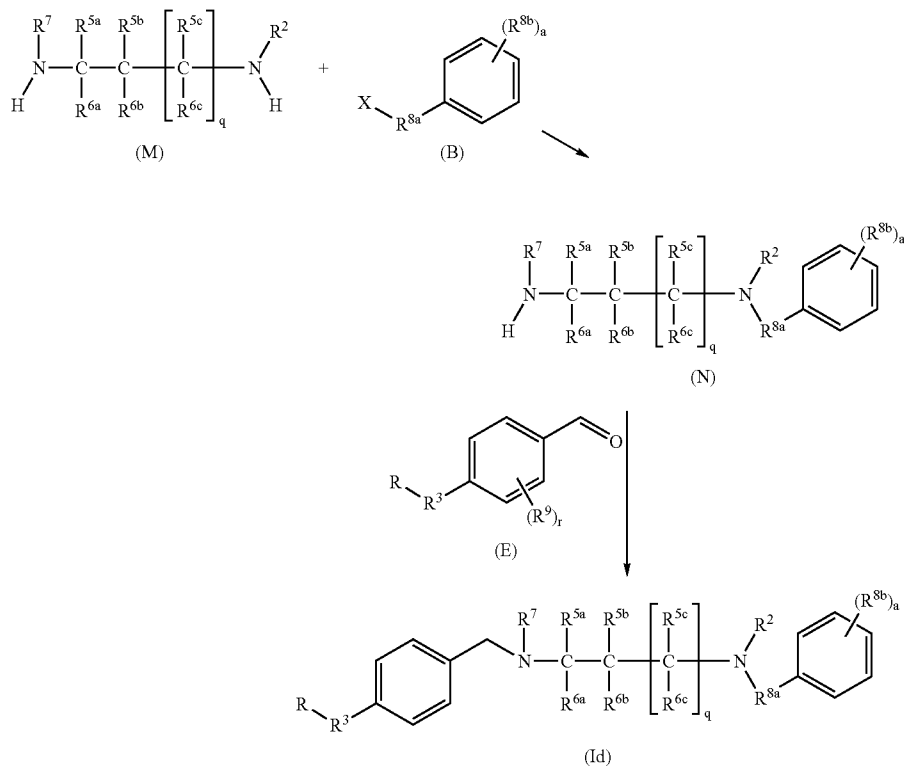
REACTION SCHEME 4
