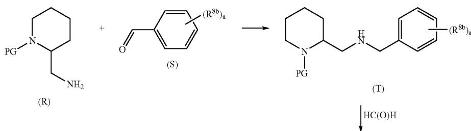
REACTION SCHEME 6
