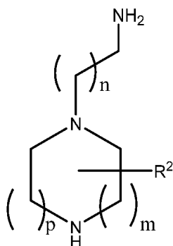
Structure II
