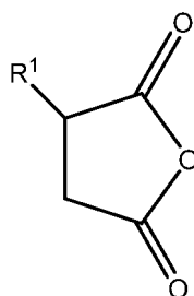
Structure I
