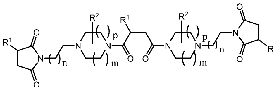
Structure III
