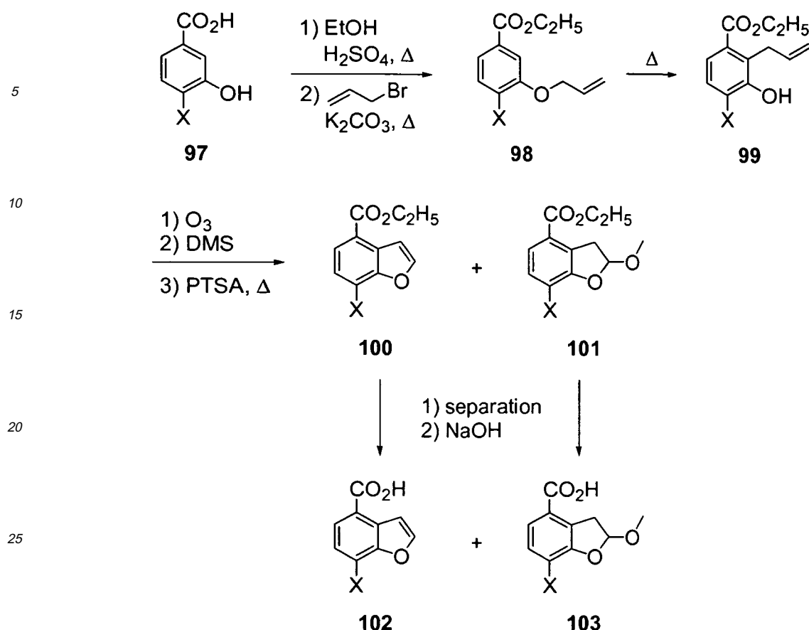
Scheme 14: Synthesis of benzofuran-carboxylic acid derivatives wherein X is fluorine or chlorine
