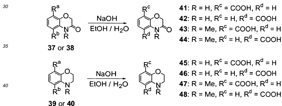
Scheme 8: Synthesis of benzo[1,4]oxazine-carboxylic acid derivatives
