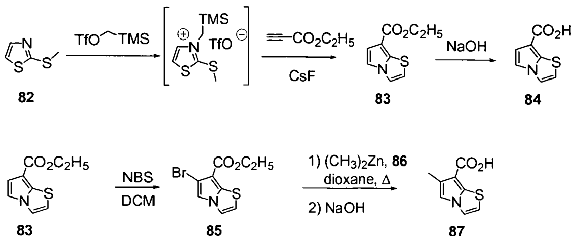
Scheme 11: Synthesis of pyrrolo[2,1-b]thiazole-carboxylic acid derivatives
