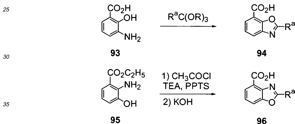
Scheme 13: Synthesis of benzoxazole-carboxylic acid derivatives wherein R is methyl or ethyl and R^a is hydrogen or methyl
