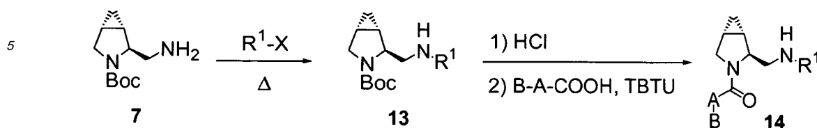
Scheme 3: Alternative synthesis of compounds of formula (I), wherein n represents 0; X represents Cl, Br, or OTf.
