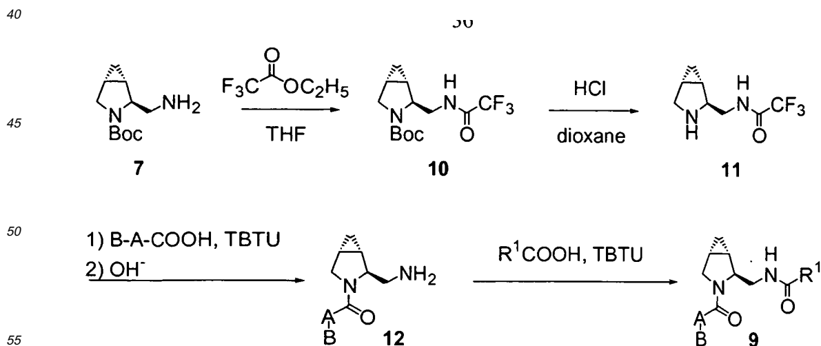
Scheme 2: Alternative synthesis of compounds of formula (I), wherein n represents 1
