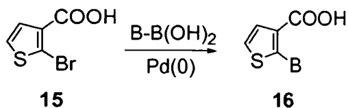
Scheme 4: Synthesis of thiophene-3-carboxylic acid derivatives
