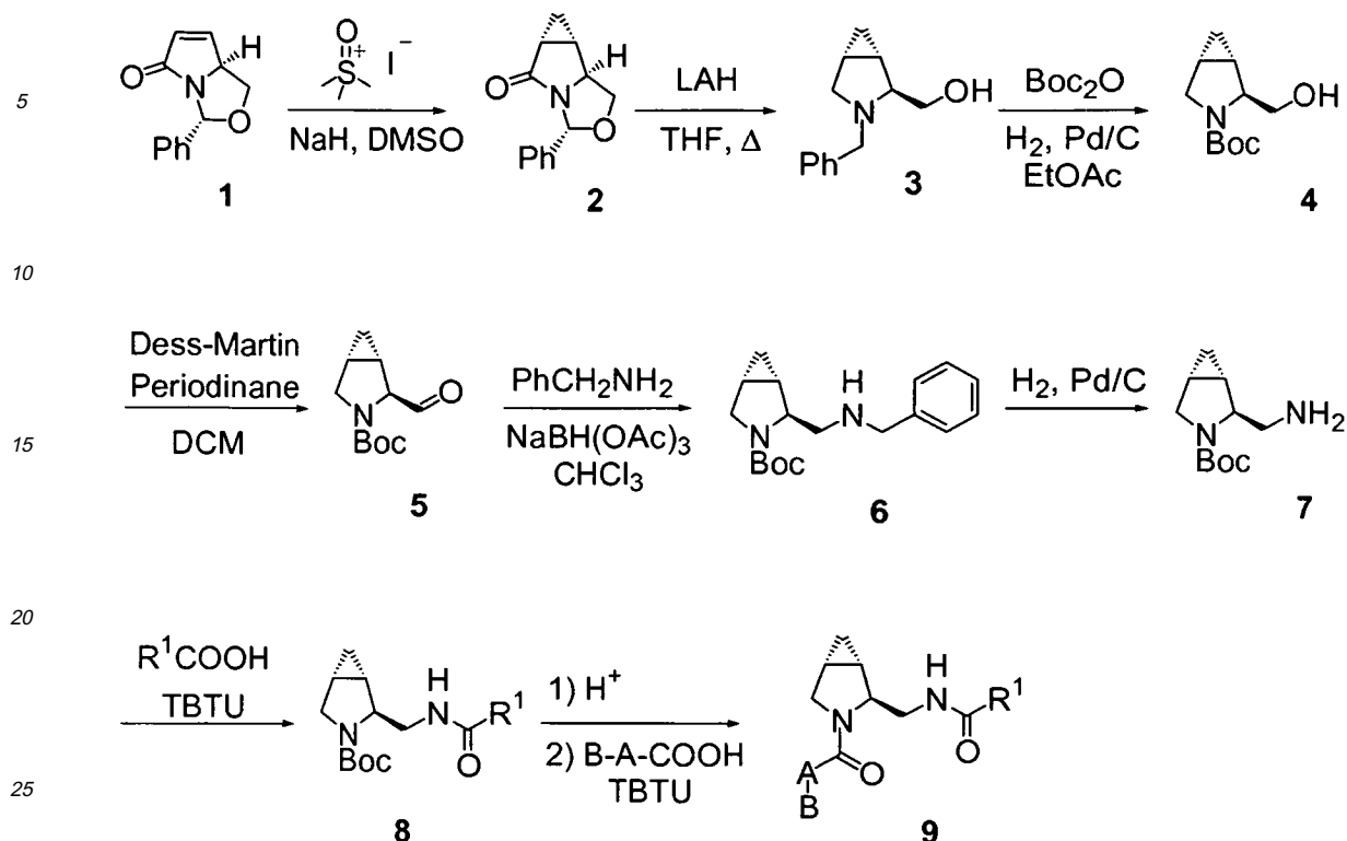
Scheme 1: Synthesis of compounds of formula (I), wherein n represents 1
