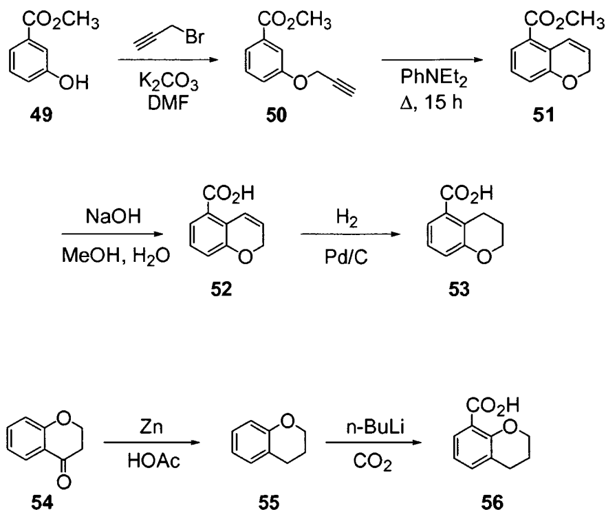
Scheme 9: Synthesis of chroman-carboxylic acid derivatives
