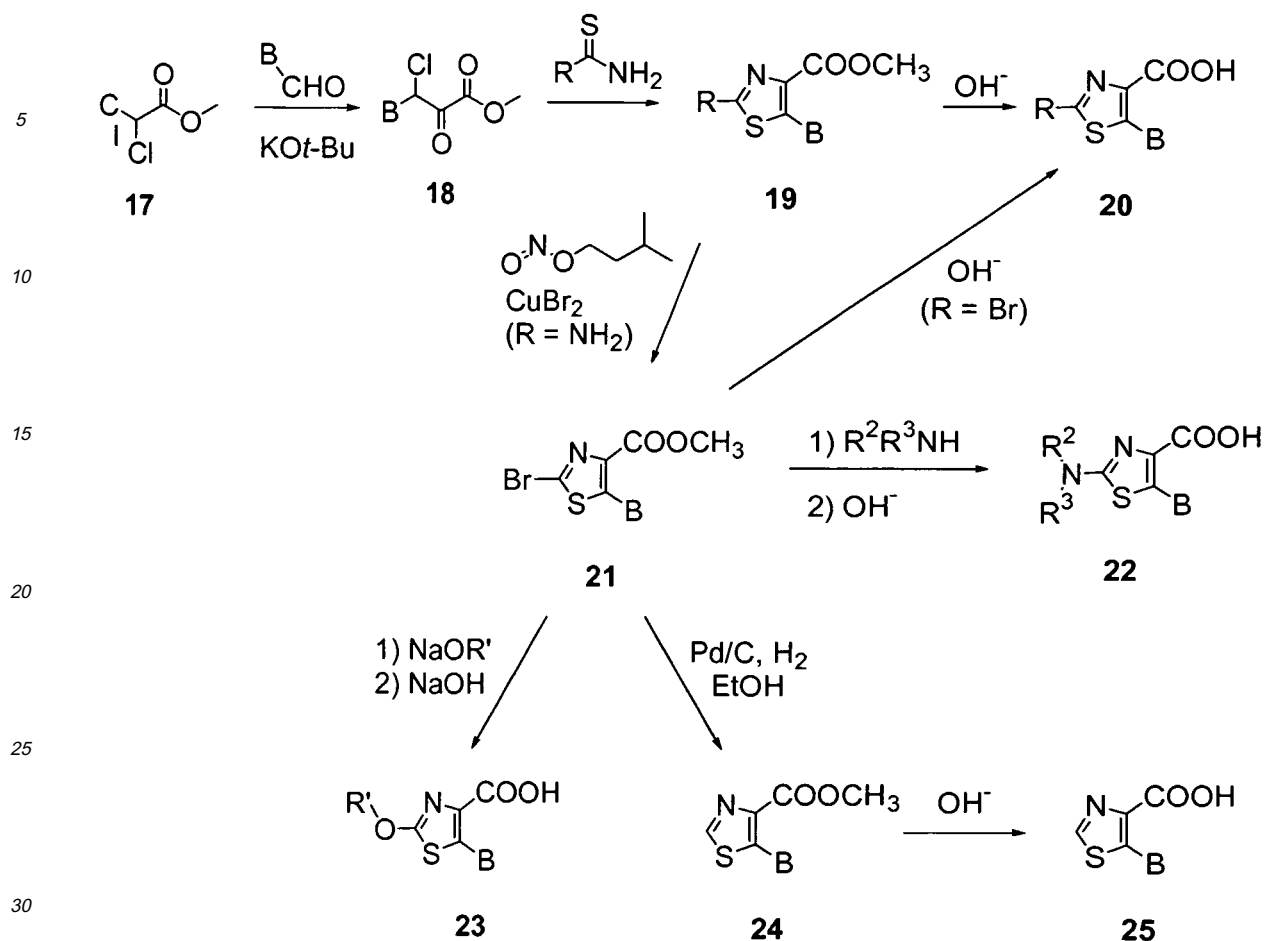
Scheme 5: Synthesis of thiazole-4-carboxylic acid derivatives, wherein
