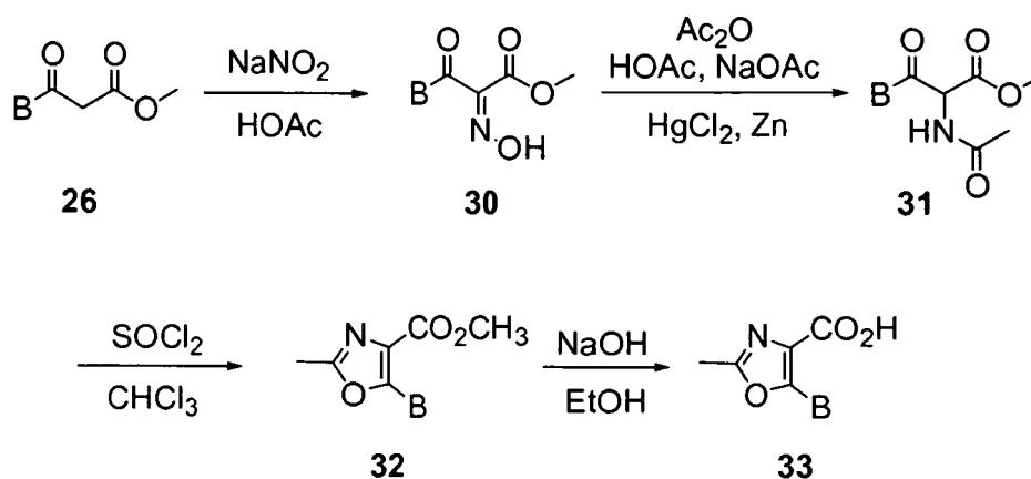
Scheme 7: Synthesis of oxazole-4-carboxylic acid derivatives
