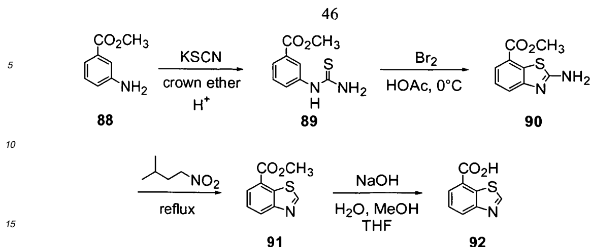
Scheme 12: Synthesis of benzothiazole-carboxylic acid derivatives
