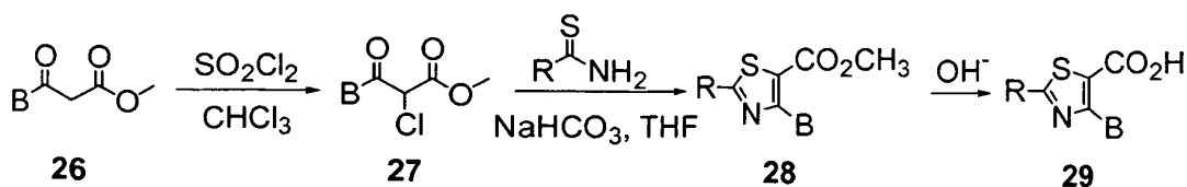
Scheme 6: Synthesis of thiazole-5-carboxylic acid derivatives, wherein R is (C 1-4 )alkyl or (C 3-6 )cycloalkyl
